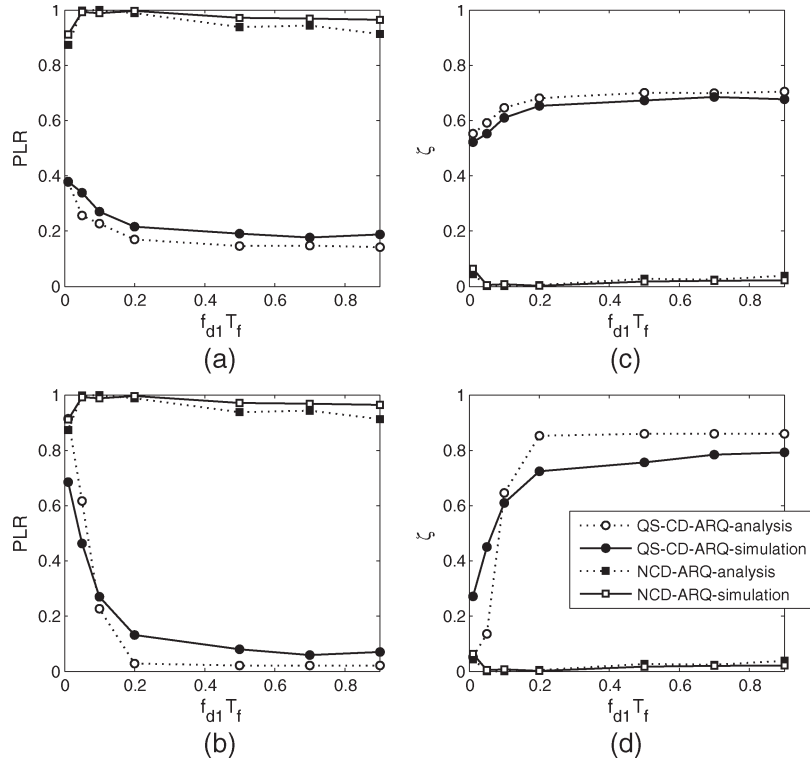
Fig. 10. PLR and throughput of the proposed scheme compared with the noncooperative scheme for various speed of the users.
