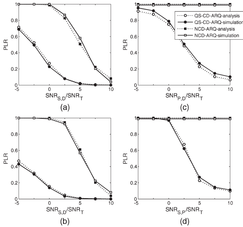
Fig. 8. PLR of the proposed scheme compared with the noncooperative scheme. [For (b), m_{P,D} is changed to 2.]
