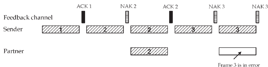
Fig. 11. DSTBC-CD-ARQ scheme (based on incremental relaying).
