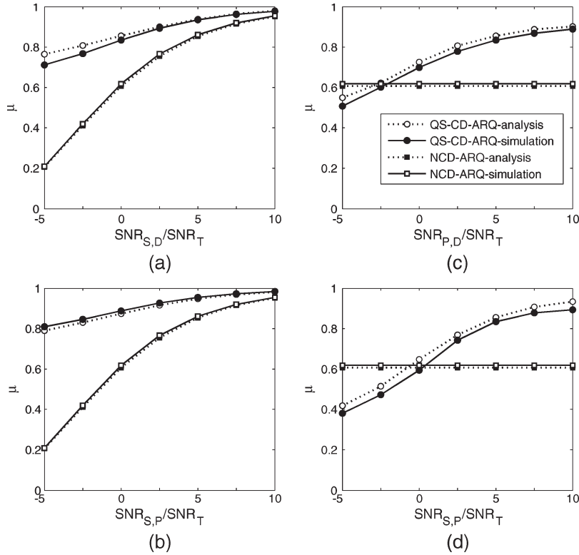
Fig. 7. Efficiency of the proposed scheme compared with the noncooperative scheme. [For (b), m_{P,D} is changed to 2.]
