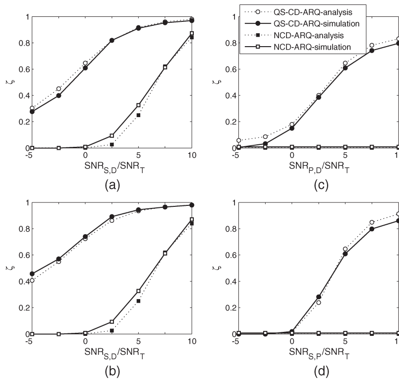
Fig. 9. Throughput of the proposed scheme compared with the noncooperative scheme. [For (b), m_{P,D} is changed to 2.]
