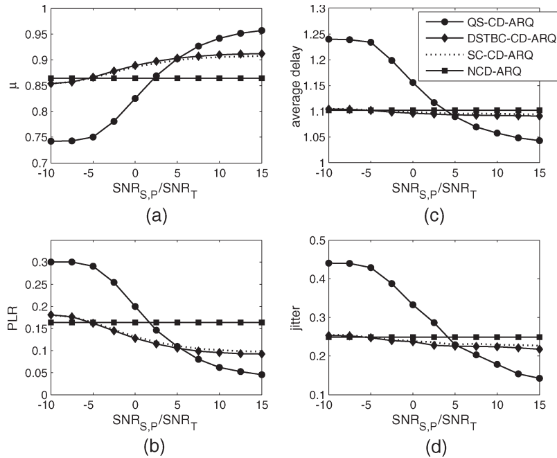
Fig. 14. Performance of the CD-ARQ scheme with varying SNR_{S,P}/SNR_T from -10 to 15 dB.
