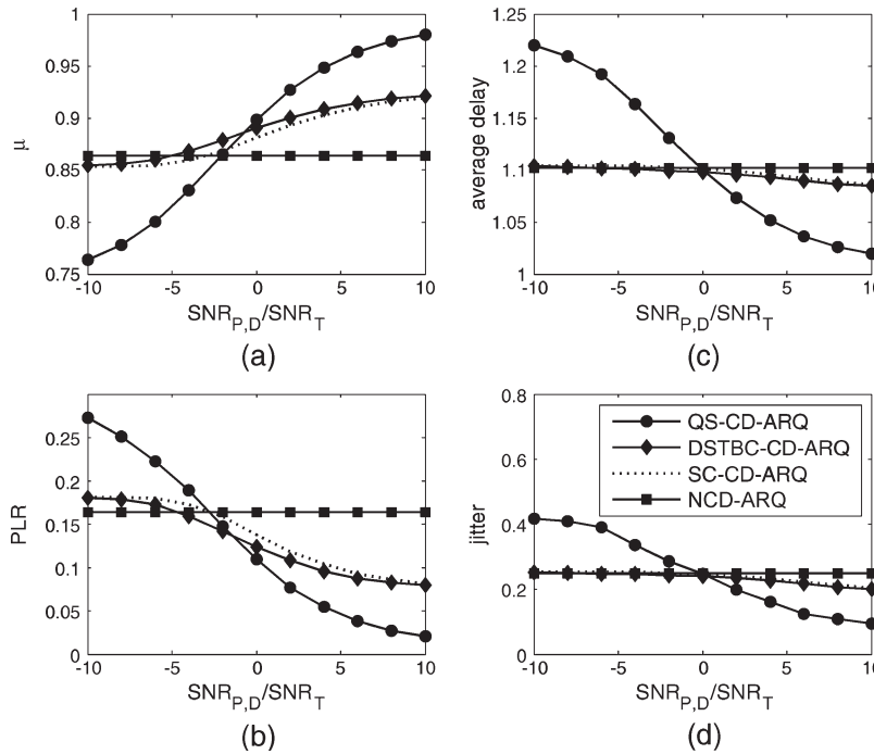
Fig. 13. Performance of the CD-ARQ scheme with varying SNR_{P,D}/SNR_T from -10 to 10 dB.
