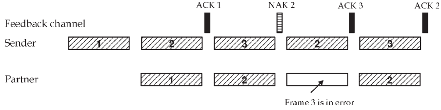
Fig. 2. QS-CD-ARQ Scheme (based on selection relaying).
