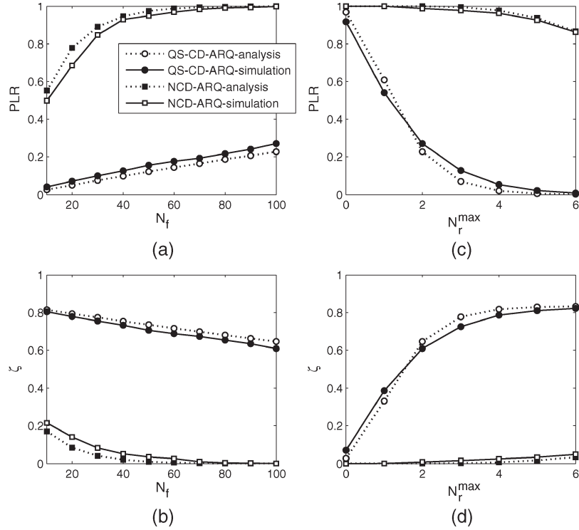
Fig. 6. PLR and throughput of the proposed scheme compared with the noncooperative scheme by varying the packet size and maximum number of retransmissions.
