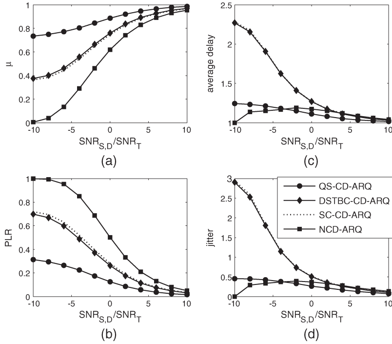
Fig. 12. Performance of the CD-ARQ scheme with varying SNR_{S,D}/SNR_T from -10 to 10 dB.
