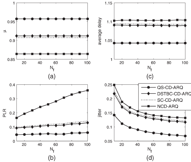
Fig. 15. Performance of the CD-ARQ scheme with varying N_f from 10 to 100 .
