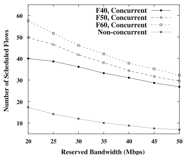
Fig. 6 Number of admitted flows vs per-flow reserved bandwidth
