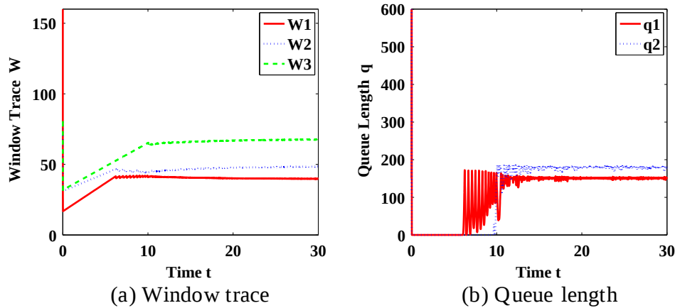
Fig. 4. Homogeneous AIMD(0.2, 0.875) flows, delay-free.
