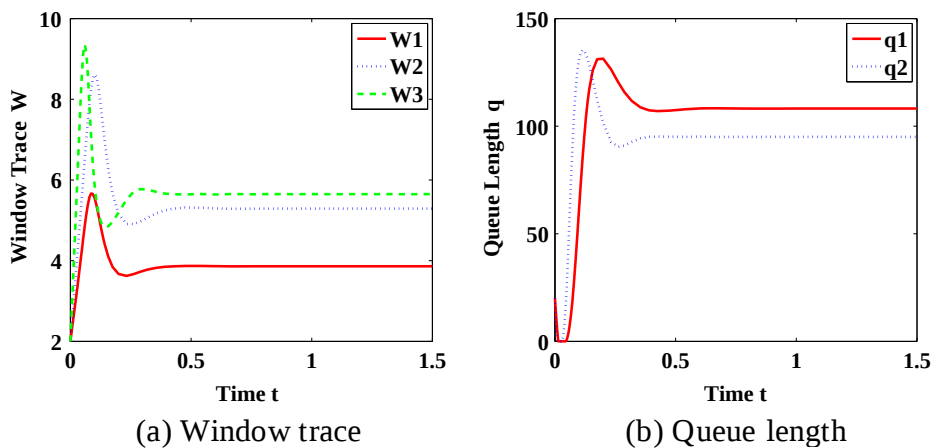
Fig. 9. Homogeneous TCP flows, with feedback delay.
