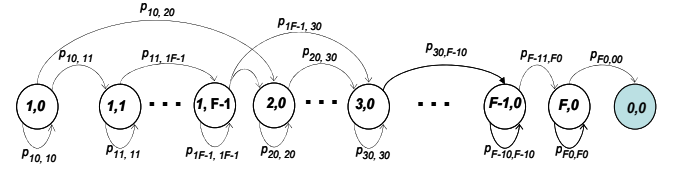
Fig. 5. The state transition diagram of the absorbing Markov chain.
