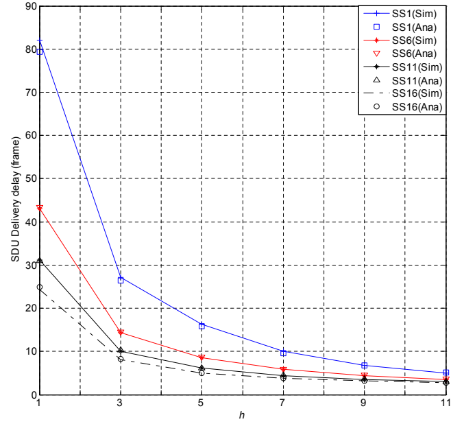
Fig. 7. The SDU delivery delay versus h .
