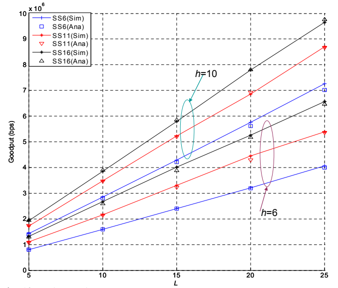
Fig. 10. The goodput versus L .
