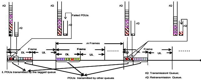
Fig. 4. The two-queue model for the delivery of SDUs.
