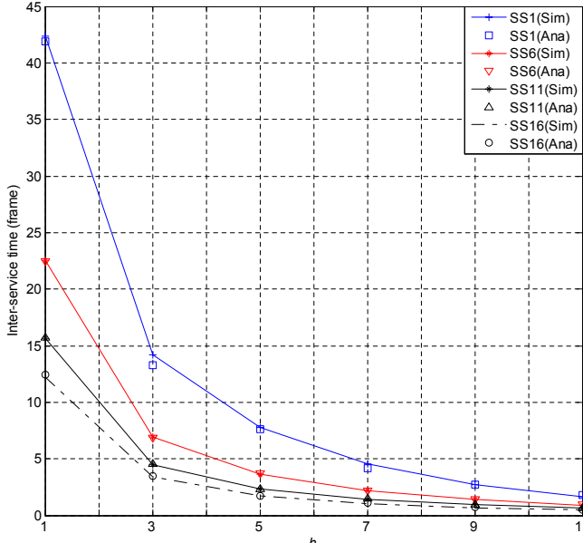
Fig. 9. The inter-service time versus h .
