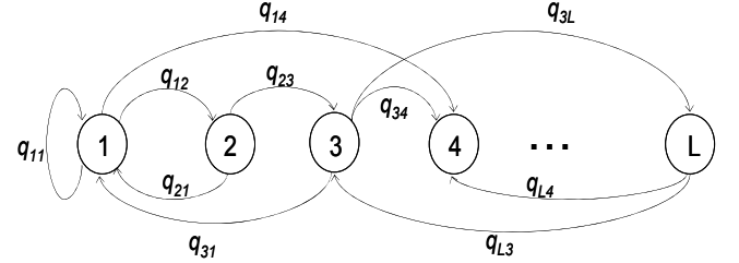
Fig. 6. The state transition diagram of HOL PDU's at the tQ queue.
