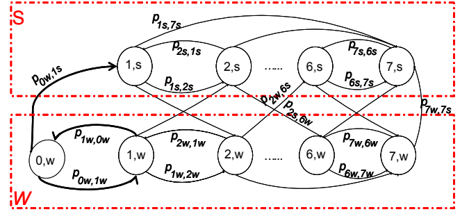
Fig. 3. The Markov model for the tagged SS.
