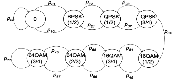
Fig. 2. Finite states Markov channel (FSMC) model.
