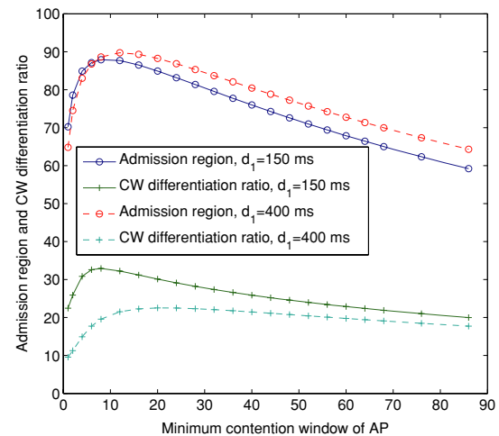
Fig. 3 The impact of the QoS requirement on the admission region when downlink flows are aggregated at the AP, with d_2 = 0 , t_{off} = 600 ms, p_{on} = 0.5
