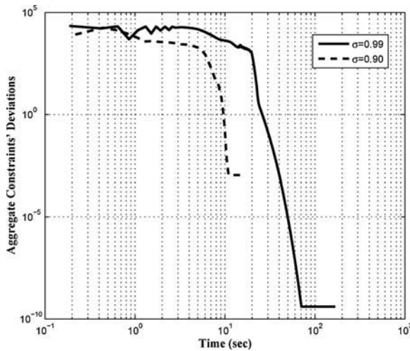
Figure 6. Aggregate penalty term constraints' deviations in PM/IPM.
