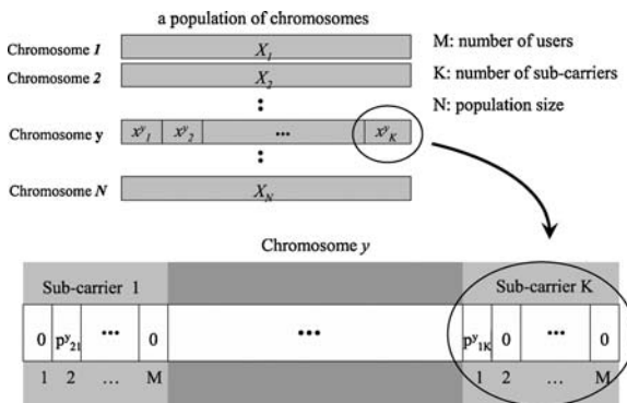
Figure 2. The population and chromosomes representations.
