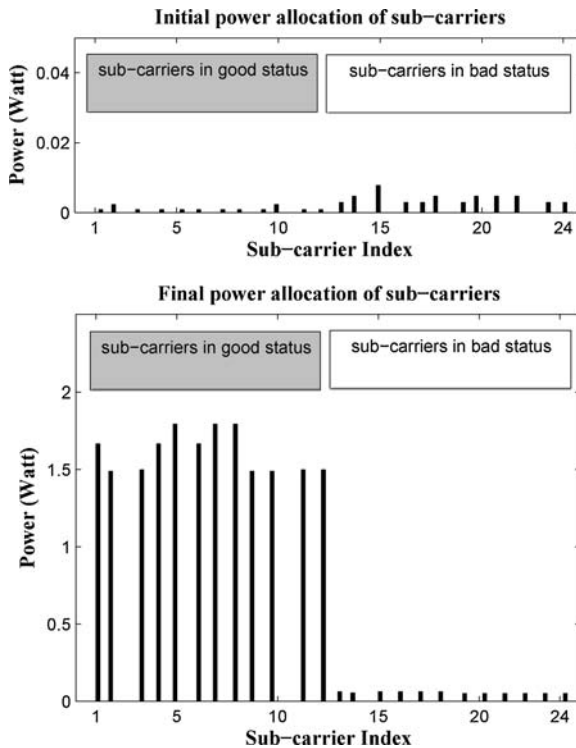
Figure 3. Power allocation distribution on sub-carriers.
