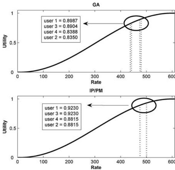
Figure 7. Utility allocation comparison of GA and PM/IPM.
