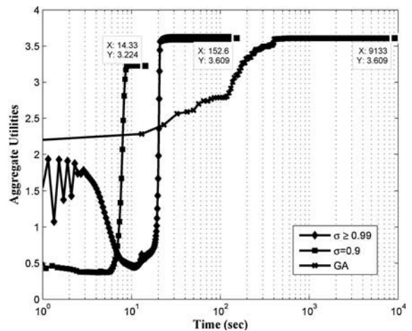
Figure 5. Convergence speed comparison of GA and PM/IPM.
