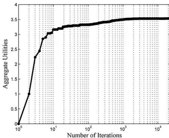
Figure 4. Convergence of fitness value.
