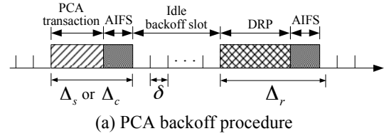
(a) PCA backoff procedure
