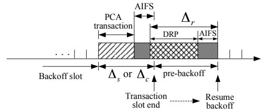
(c) Pre-backoff waiting in hybrid MAC
