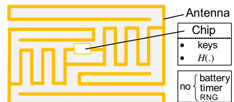
Fig. 3. Architecture of a passive RFID tag under consideration.
