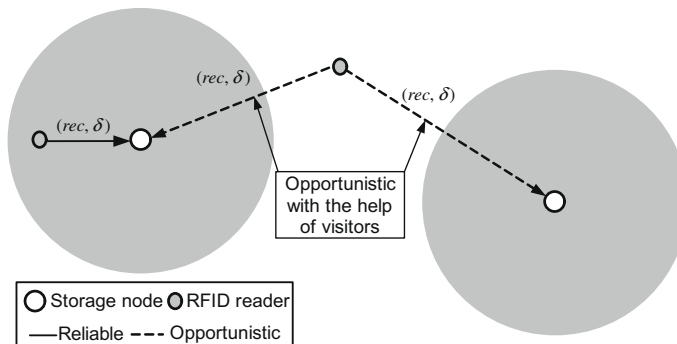
Fig. 5. Opportunistic tag information aggregation in MCMD policy.
