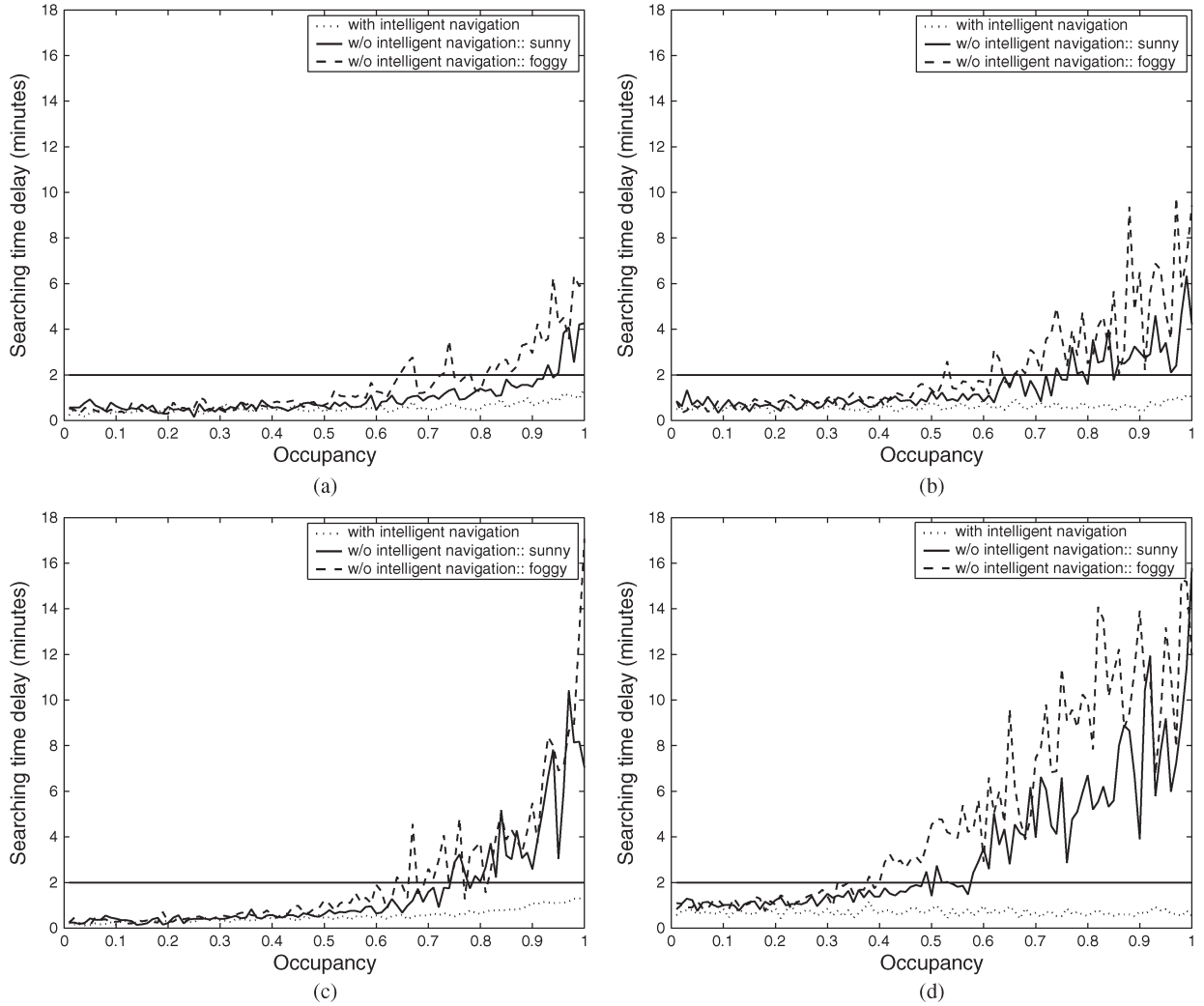
Fig. 8. Occupancy factor of parking lot versus the STD. (a) p = 10\% . (b) p = 30\% . (c) p = 50\% . (d) p = 80\% .
