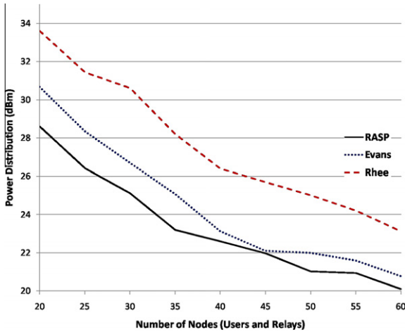
Fig. 9. Comparison of power distribution over varying number of nodes.
