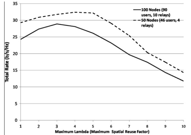
(a) 256 subcarriers
