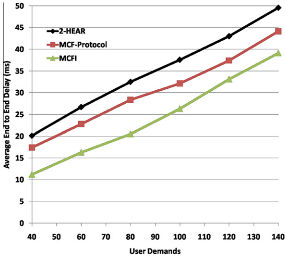
Fig. 5. End-to-end delay comparison for networks with 47 nodes (1 BS, 6 relays and 40 users).
