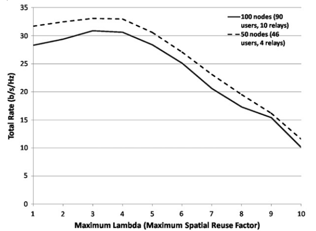
(b) 512 subcarriers
