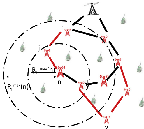
Fig. 3. Illustration of the subcarrier allocation interference constraint.
