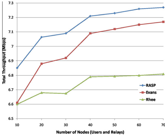
Fig. 8. Total throughput versus the number of nodes.
