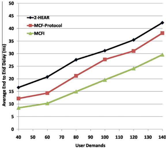
Fig. 6. End-to-end delay comparison for networks with 25 nodes (1 BS, 4 relays and 20 users).
