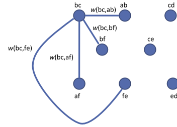
(b) Composition of weighted conflict graph, WCG, for link (b, c)
