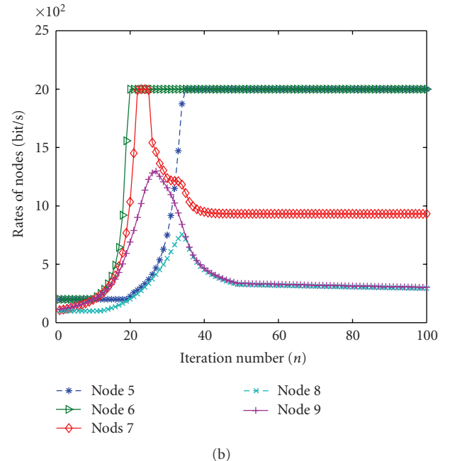
FIGURE 5: Convergence of the ASMOP algorithm by using hierarchical sequence method.
