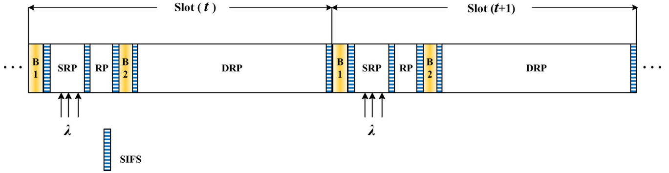
Fig. 1. Slotted-time structure of the CC Channel.
