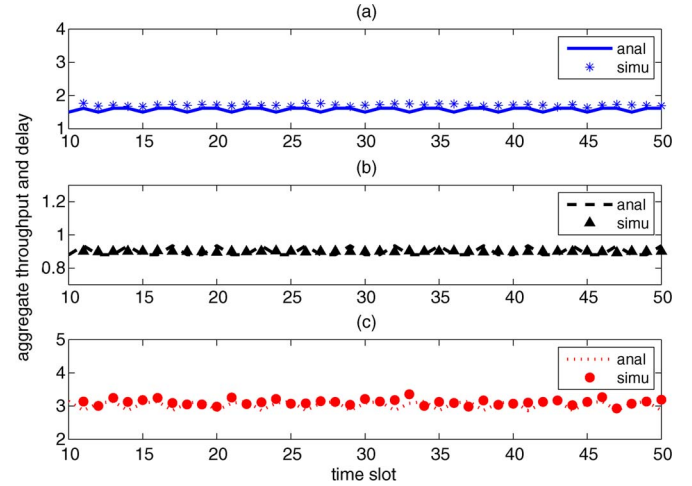
Fig. 6. Average (a) user aggregate throughput \bar{S} (in channels per user), (b) network normalized aggregate throughput \bar{\Theta} , and (c) user delay \bar{D} (in time slots) for a number of time slots when T_{res} = 3 (ms) and \lambda_{ad} = 3 (user/ms).
