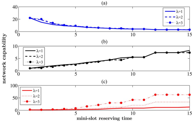
Fig. 7. Effects of the minislot reserving time T_{res} (in milliseconds) on the network capability. (a) Average number of admitted users \bar{M}_{aw} . (b) User average aggregate throughput \bar{S} (in channels per user). (c) User average delay \bar{D} (in time slots).
