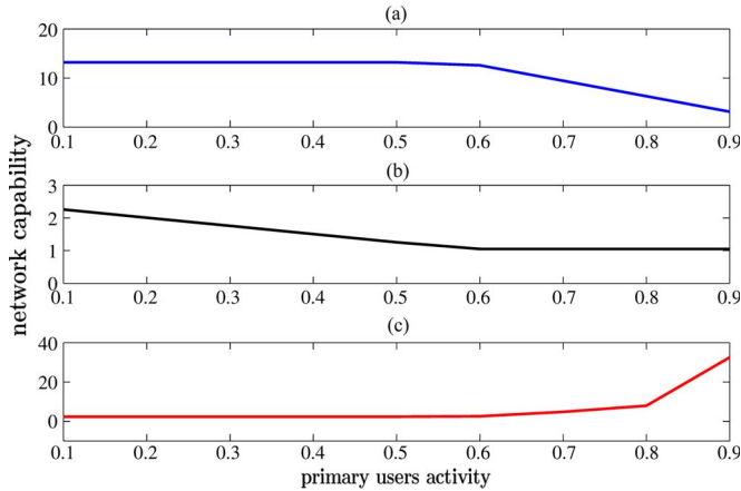
Fig. 11. Effects of the primary user activity \delta on the network capability when T_{res} = 3 (ms) and \lambda_{ad} = 2 (user/ms). (a) Average number of admitted users \bar{M}_{aw} . (b) User average aggregate throughput \bar{S} (in channels per user). (c) User average delay \bar{D} (in time slots).
