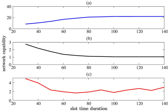
Fig. 10. Effects of the slot time duration T (in milliseconds) on the network capability when T_{res} = 3 (ms) and \lambda_{ad} = 2 (user/ms). (a) Average number of admitted users \bar{M}_{aw} . (b) User average aggregate throughput \bar{S} (in channels per user). (c) User average delay \bar{D} (in time slots).
