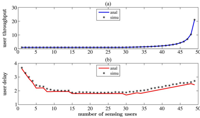
Fig. 4. SU's (a) average aggregate throughput, \bar{S} (in channels per user) and (b) average waiting delay \bar{D} (in time slots) with respect to the number of sensing users M_s at a time slot when M_{B1} = 50 (users), \lambda_{ad} = 1 (user/ms), and T_{res} = 2 (ms).
