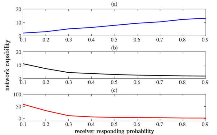
Fig. 9. Effects of the receiver responding probability p on the network capability when T_{res} = 3 (ms) and \lambda_{ad} = 2 (user/ms). (a) Average number of admitted users \bar{M}_{aw} . (b) User average aggregate throughput \bar{S} (in channels per user). (c) User average delay \bar{D} (in time slots).
