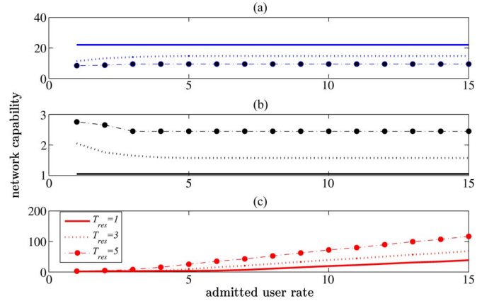
Fig. 8. Effects of the admitted user rate \lambda_{ad} (in users per milliseconds) on the network capability. (a) Average number of admitted users \bar{M}_{aw} . (b) User average aggregate throughput \bar{S} (in channels per user). (c) User average delay \bar{D} (in time slots).
