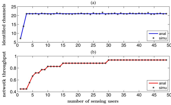
Fig. 3. Relation between the number of sensing users M_s and (a) the number of identified licensed channels N_a and (b) the network normalized average aggregate throughput \bar{\Theta} in a time slot when M_{B1} = 50 (users), \lambda_{ad} = 1 (user/ms), and T_{res} = 2 (ms).
