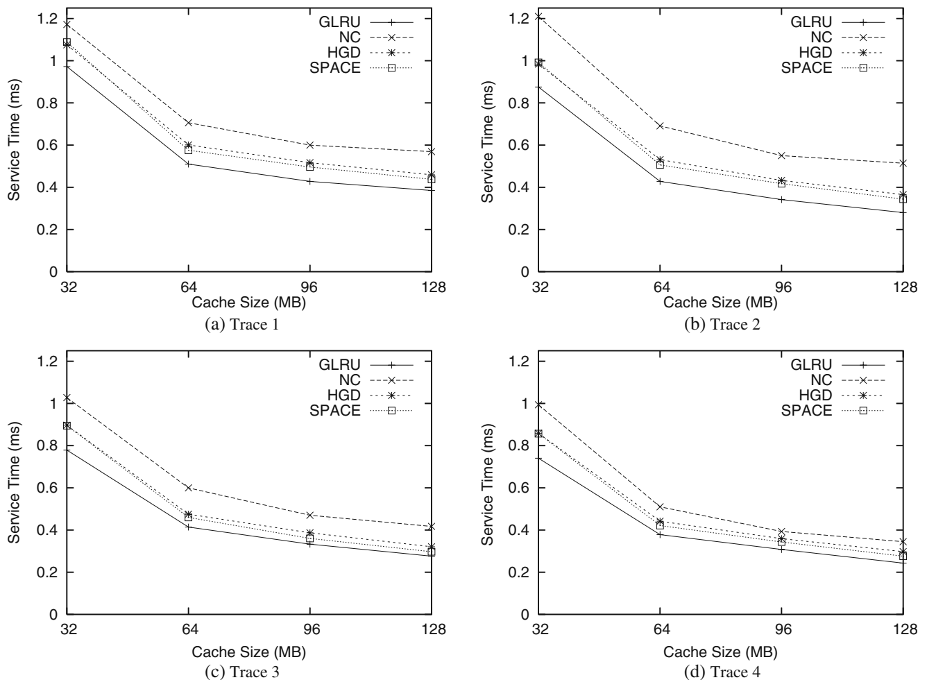
Fig. 3 Service time for different traces (a–d)
