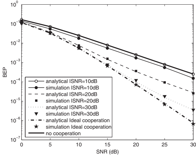
Fig. 5. Bit error probability of the CD system with 4-QAM/QPSK for similar channel towards BS.
