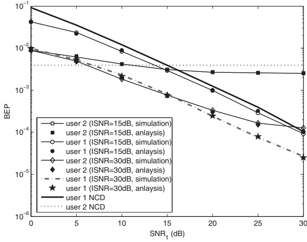
Fig. 2. Bit error probability of the CD system with 4-QAM/QPSK for dissimilar channel towards BS ( SNR_2 = 15dB ).
