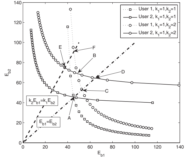
Fig. 7. E_{b1} vs E_{b2} of both user 1 and user 2 for various channel conditions ( e_1 = e_2 = 1 \times 10^{-3} ).
