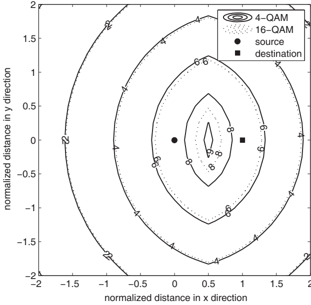
Fig. 10. Cooperative regions of the CD system with ESR at BS for various G_{cd} of the sender ( e_1 = e_2 = 1 \times 10^{-3} ).
