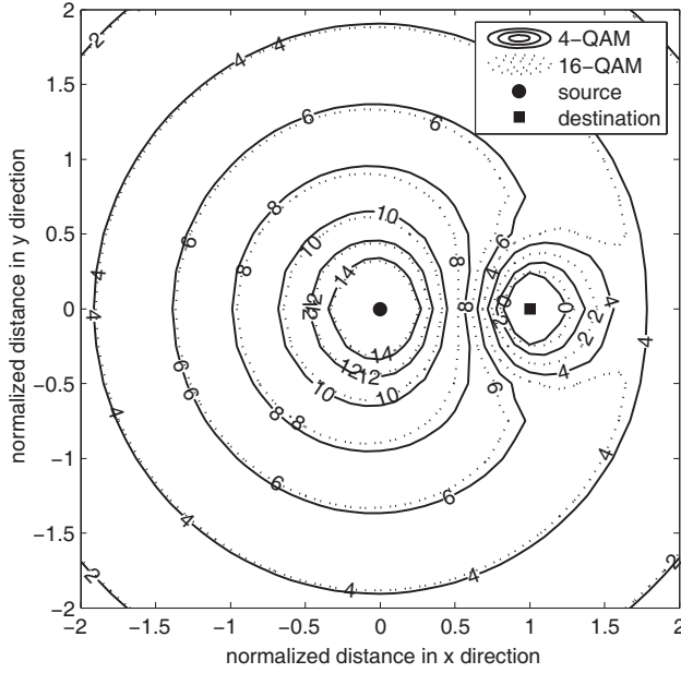
Fig. 8. Cooperative regions of the CD system with OPA mechanism for various G_{cd} of the sender ( e_1 = e_2 = 1 \times 10^{-3} ).
