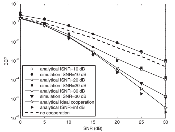
Fig. 6. Bit error probability of the CD system with 16-QAM for similar channel towards BS.
