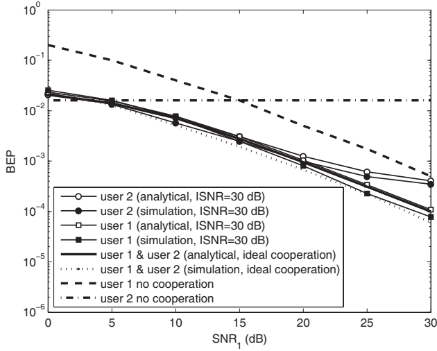
Fig. 4. Bit error probability of the CD system with 16-QAM for dissimilar channel towards BS ( SNR_2 = 30dB ).
