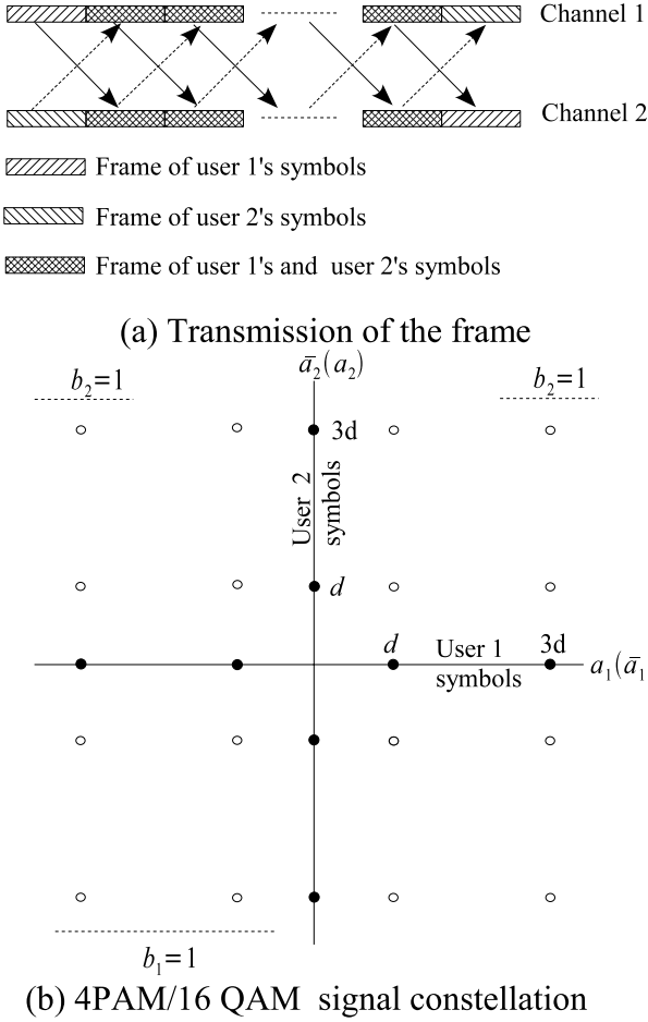
Fig. 1. (a) Frame transmission format and (b) signal constellation of 4-PAM/16-QAM using quadrature signaling.
