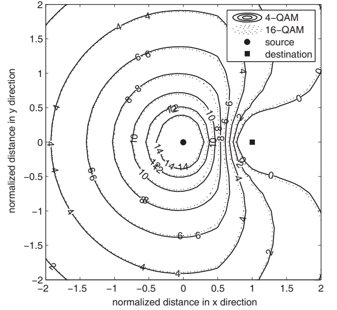
Fig. 9. Cooperative regions of the CD system with EPT for various G_{cd} of the sender ( e_1 = e_2 = 1 \times 10^{-3} ).
