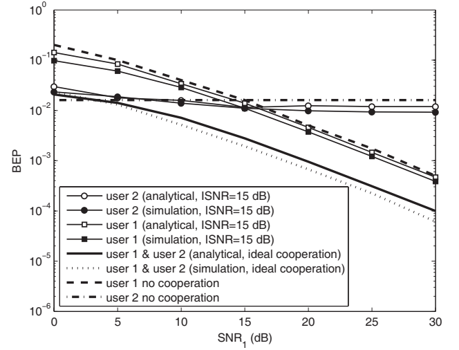
Fig. 3. Bit error probability of the CD system with 16-QAM for dissimilar channel towards BS ( SNR_2 = 15dB ).
