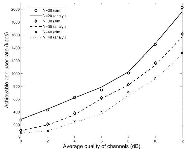
Fig. 12. Achievable per-user rate versus the average quality of wireless channels for an unsaturated case.
