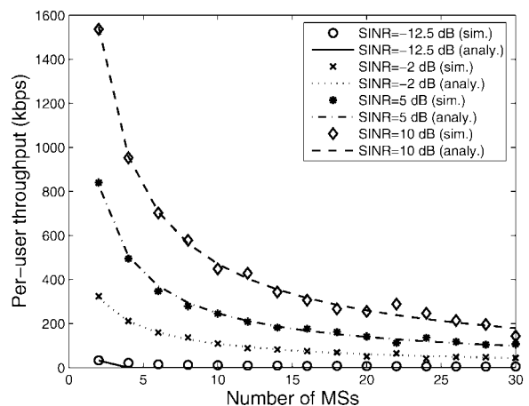
Fig. 8. Achievable per-user rate versus the number of users for a saturated case (the second model).
