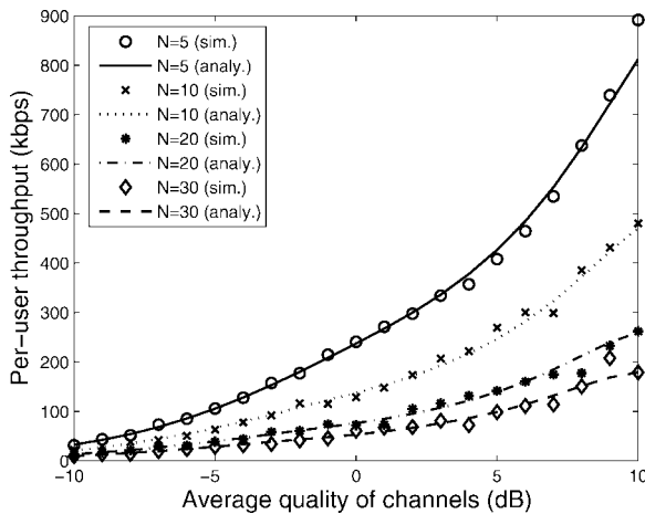
Fig. 9. Achievable per-user rate versus the average quality of wireless channels for a saturated case (the second model).
