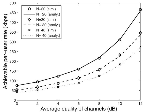
Fig. 7. Achievable per-user rate versus the average quality of wireless channels for a saturated case (the first model).
