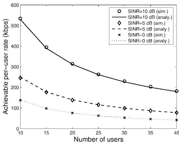
Fig. 6. Achievable per-user rate versus the number of users for a saturated case (the first model).
