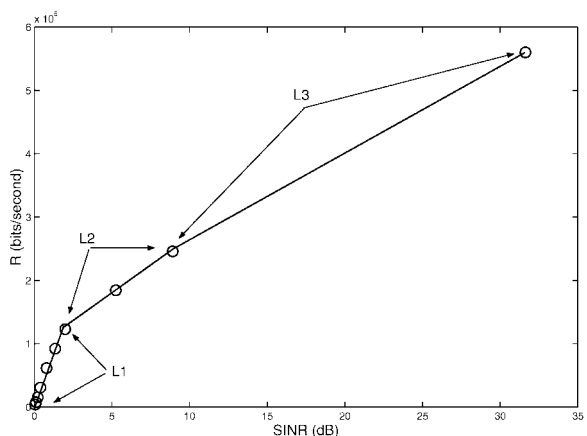
Fig. 3. Piecewise linear modeling of the achievable rates versus SINR values.
