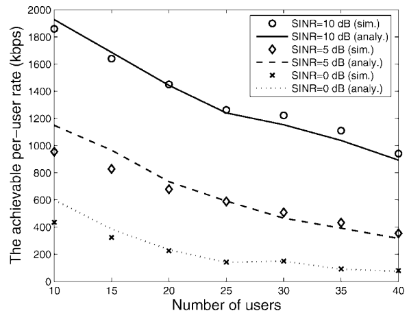
Fig. 11. Achievable per-user rate versus the number of users for an unsaturated case.
