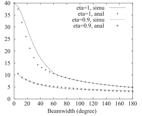
Fig. 6. Number of concurrent transmissions, case 4.
