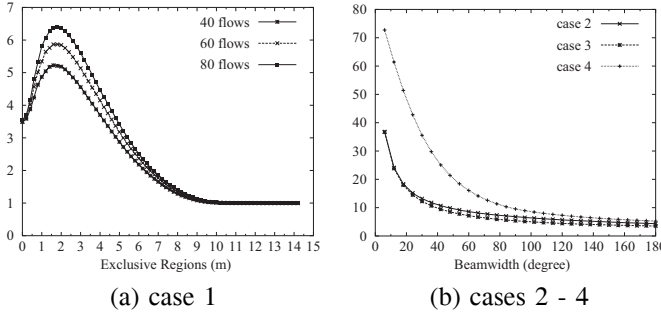
Fig. 5. Spatial multiplexing gain.
