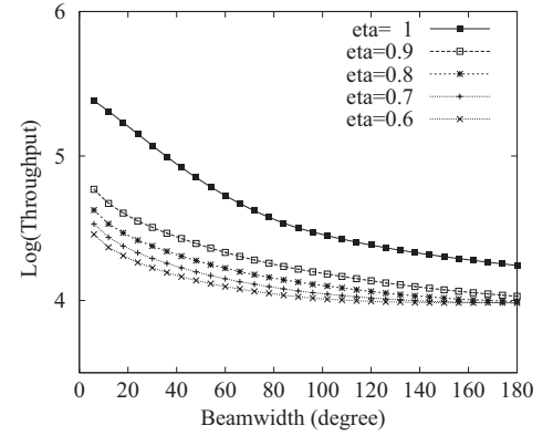
Fig. 7. Throughput with different antenna efficiency, case 4.
