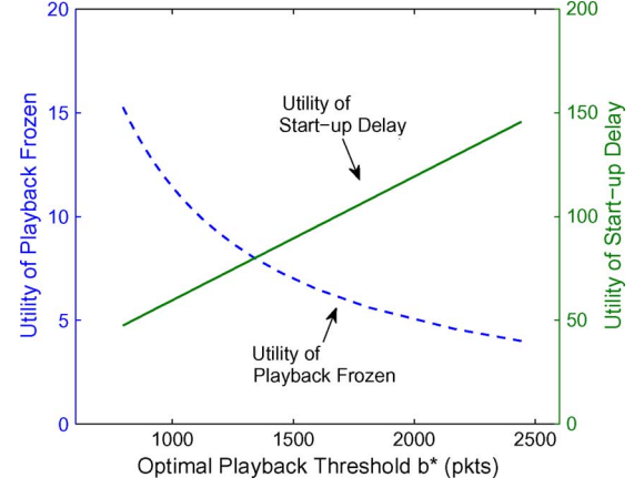
Fig. 10. Trade-off between the number of playback freezes and start-up delay at different optimal playback thresholds b^* .
