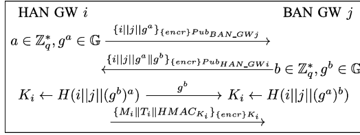
Fig. 4. Proposed lightweight message authentication scheme.
