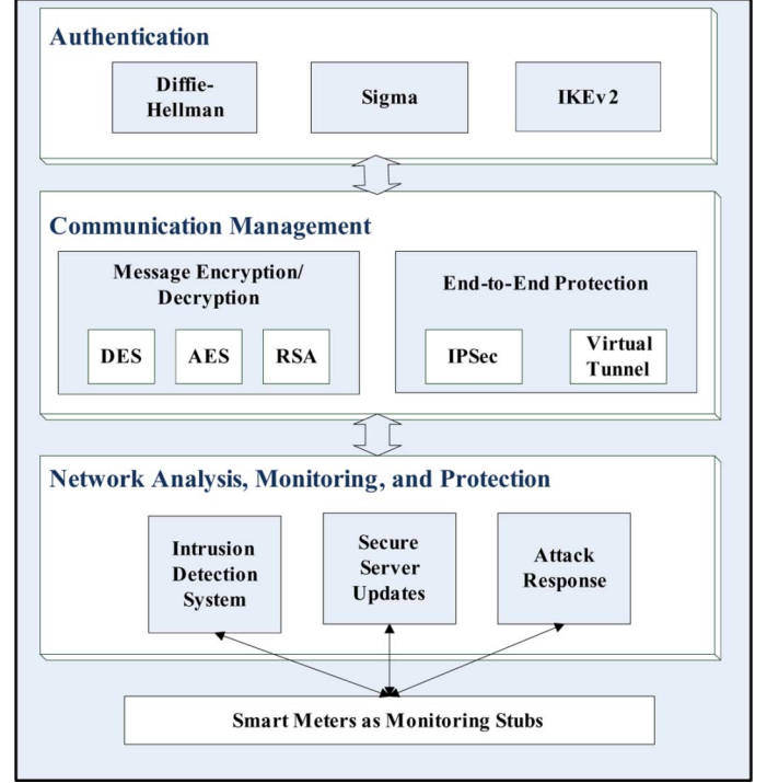
Fig. 3. Envisioned security framework for SG communications.
