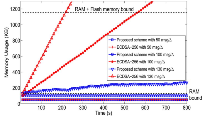
Fig. 7. Memory usage of the proposed and conventional ECDSA authentication algorithms for different message volumes received by BAN.
