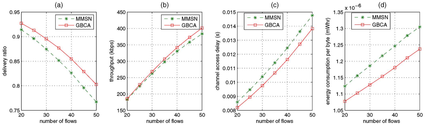
Fig. 9. Performance comparison between GBCA and MMSN with number of flows increasing in non-tree/forest routing scenario.
