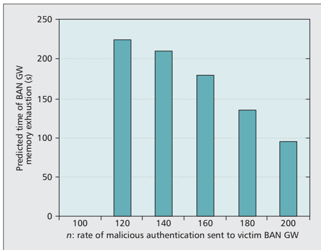
Figure 4. Predicted time of BAN GW memory exhaustion by the proposed algorithm for shorter training time of 50 s in case of different DDoS attack rates.
