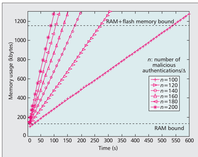
Figure 2. Memory usage of the victim BAN GW over time for various rates of malicious authentication requests.
