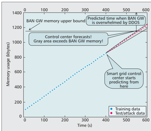
Figure 3. Obtaining prediction time using the proposed forecasting method.
