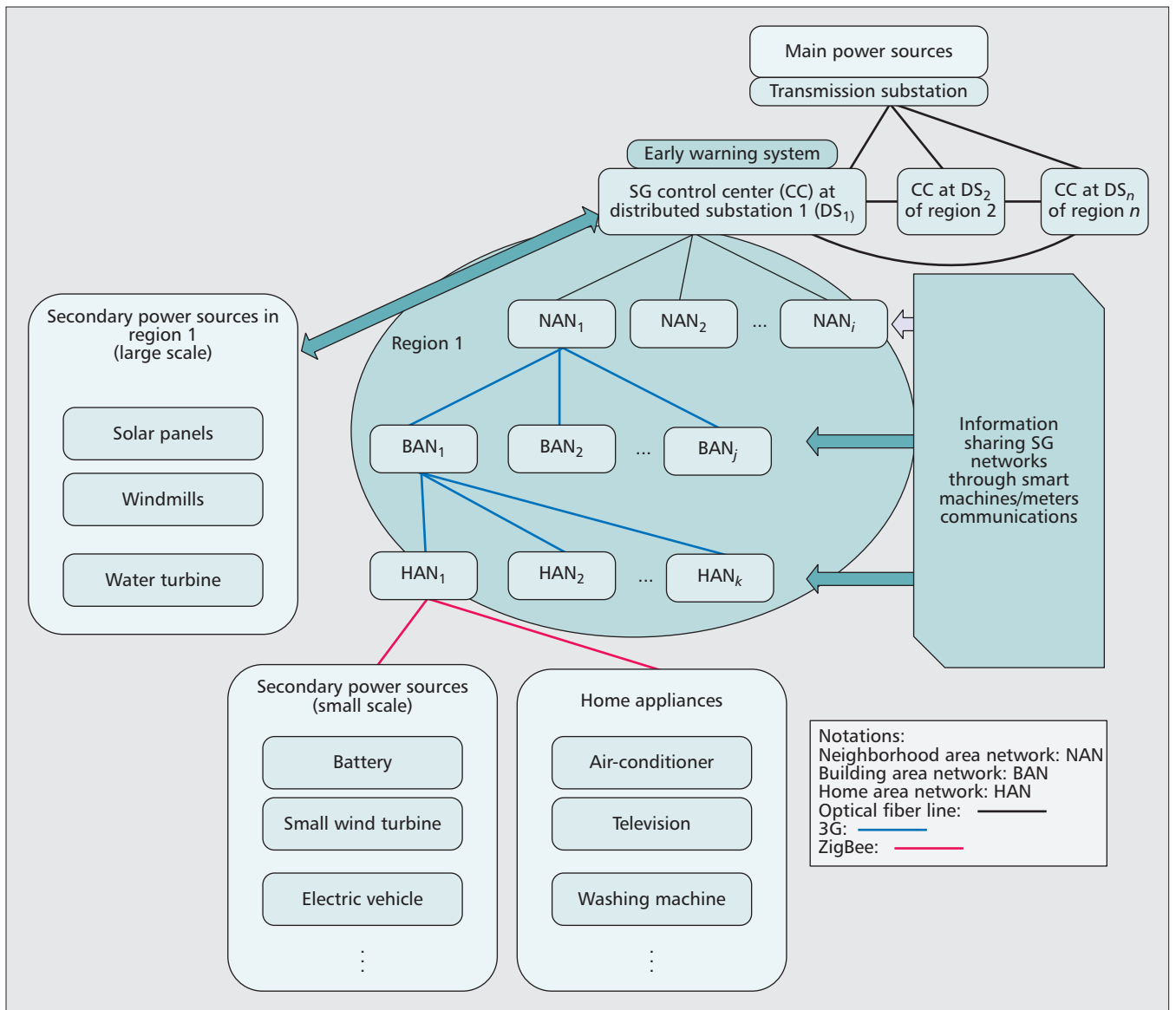
Figure 1. Smart grid hierarchical networks.
