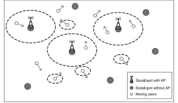
Fig. 3. Network model.
