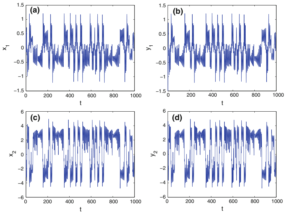
Fig. 9 State trajectories of the master system ( left ) and the slave system ( right ) in IIS.
