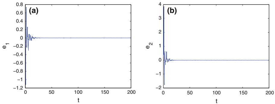
Fig. 8 Synchronization errors in GISS: a e_1(t) and b e_2(t) with \Delta_{k,i} = 1.0 and B_k = 0.90I .
