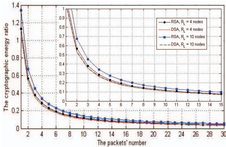
Fig. 15: The ratio of ESIP's cryptographic energy to that of signature-based protocol.
