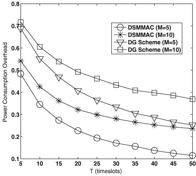
Fig. 9. Power consumption overhead versus the duration of each data transmission.
