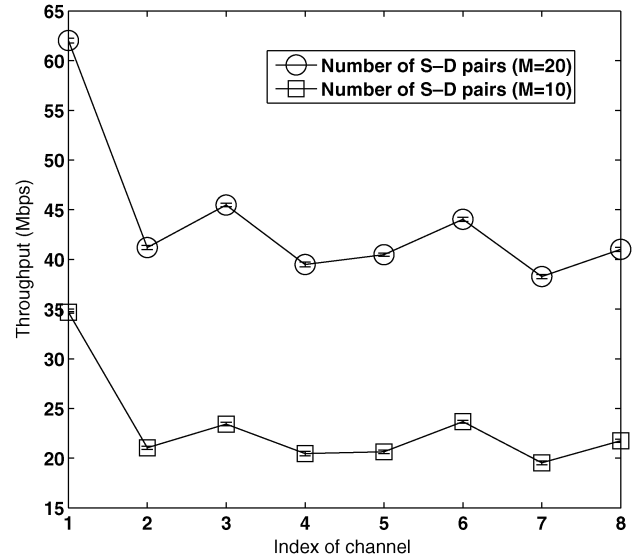
Fig. 8. Achieved throughput over each channel.
