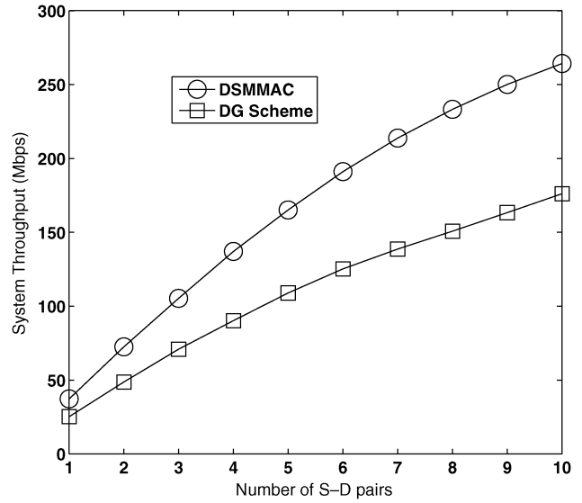
Fig. 10. System throughput with different numbers of S-D pairs.
