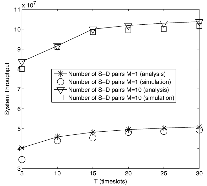
Fig. 4. System throughput versus the duration of each data transmission.
