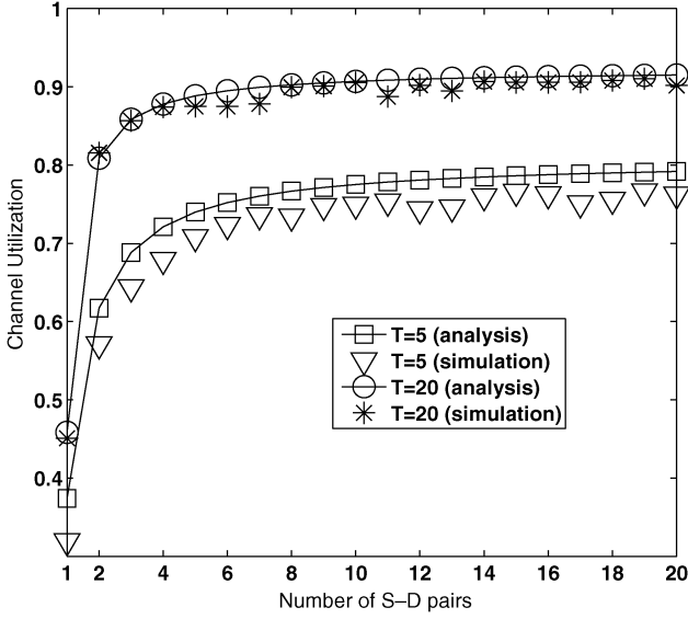
Fig. 5. Channel utilization with different numbers of S-D pairs.
