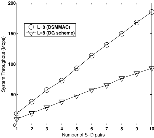
Fig. 6. System throughput with different numbers of S-D pairs.
