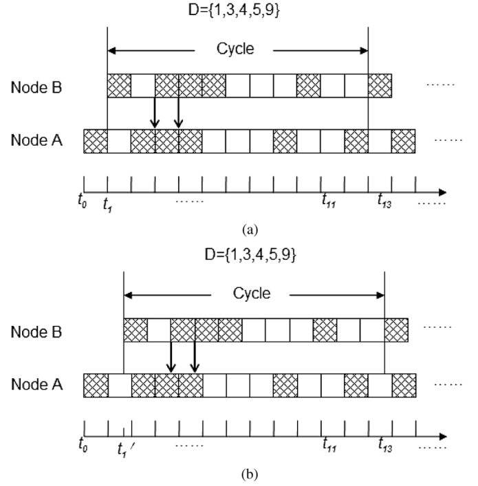
Fig. 2. Rotation closure property for the difference set D = \{1, 3, 4, 5, 9\} . (a) Aligned boundaries of time slots. (b) Nonaligned boundaries of time slots.
