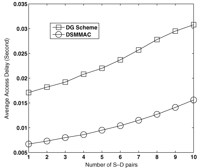
Fig. 11. Medium access delay with different numbers of S-D pairs.
