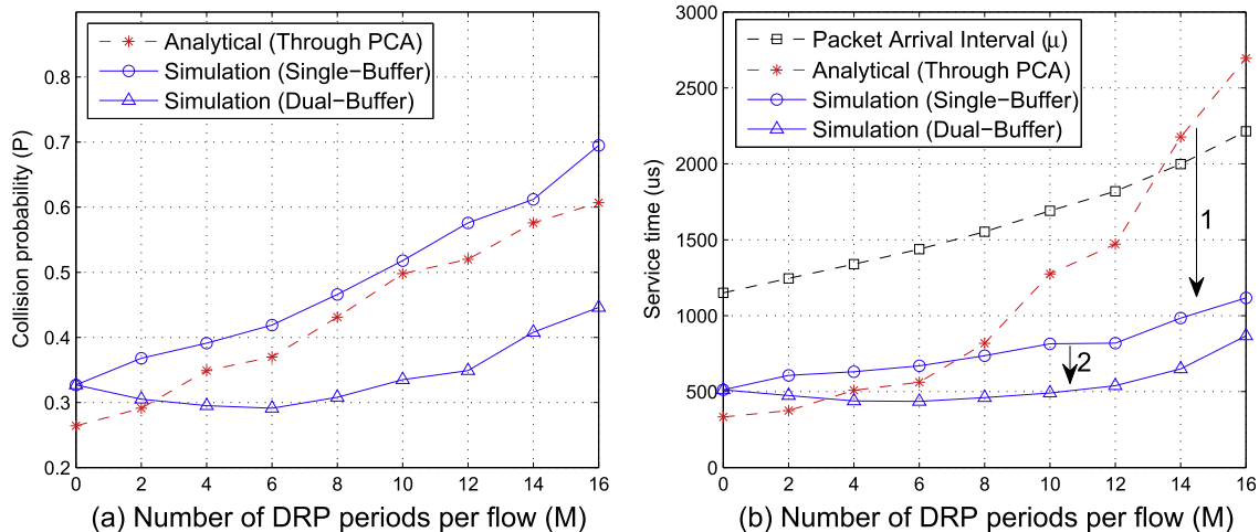
Fig. 6. Performance vs. M for video streaming.
