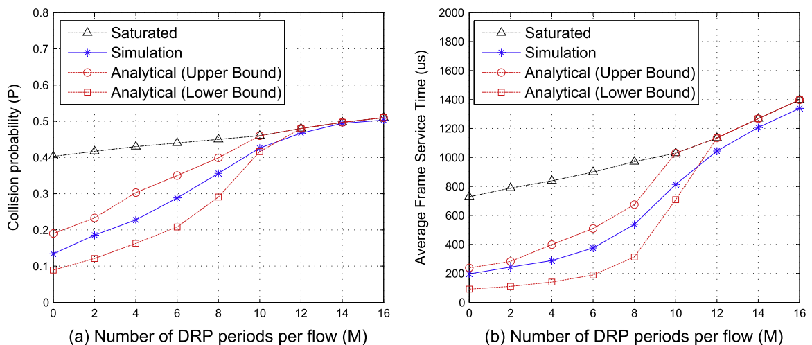
Fig. 4. Performance vs. M for unsaturated PCA stations.
