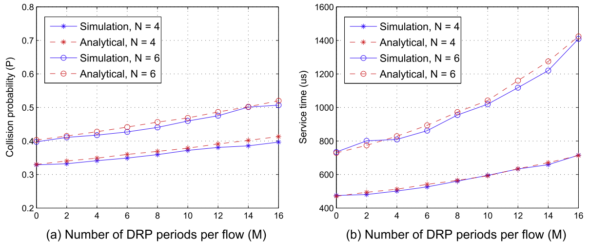
Fig. 3. Performance vs. M for saturated PCA stations.
