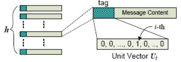
Fig. 5. Packet tagging before source encoding.
