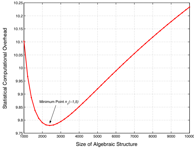
Fig. 9. Computational overhead vs. size of algebraic structure ( t=5 ).
