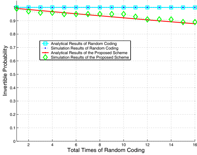
Fig. 8. Invertible probability vs. total times of random coding ( p=241 , q=251 ).
