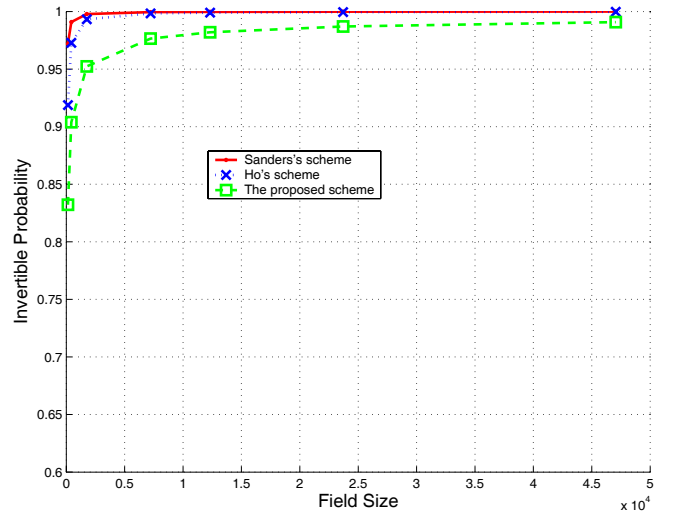
Fig. 7. Invertible probability vs. field size (theoretical analysis).
