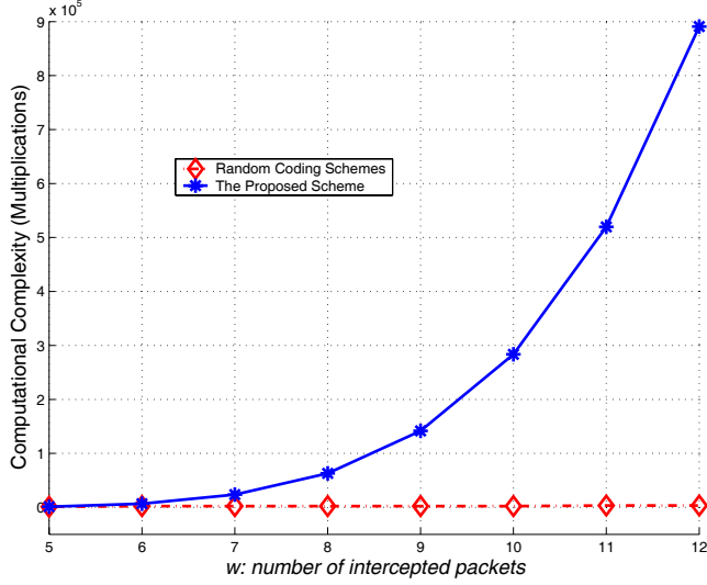
Fig. 6. Privacy enhancement in terms of the order of computational complexity ( h=5 , l=200 ).
