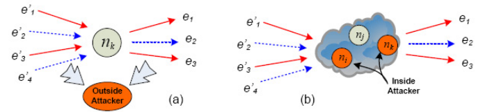
Fig. 3. Attack model: (a) outside attacker; (b) inside attacker.
