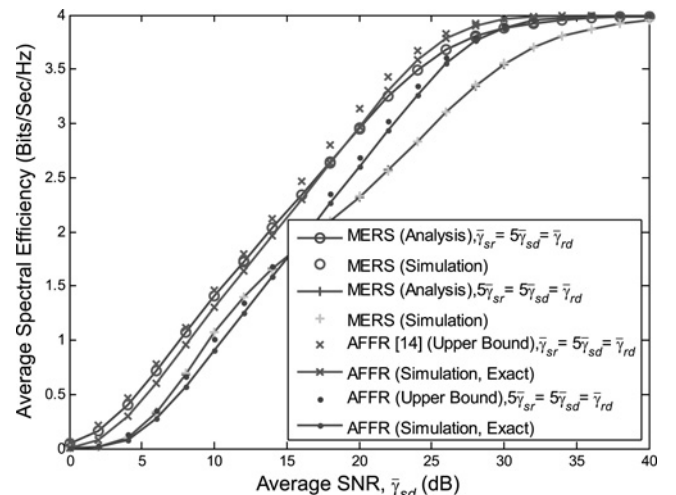
Fig. 3 Average spectral efficiency of the MERS
