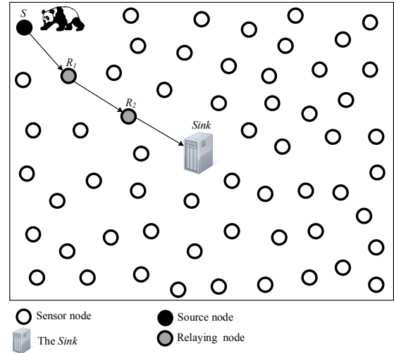
Fig. 1: The architecture of the considered WSN.
