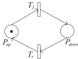
Fig. 2. The failure-repair model of a single component
