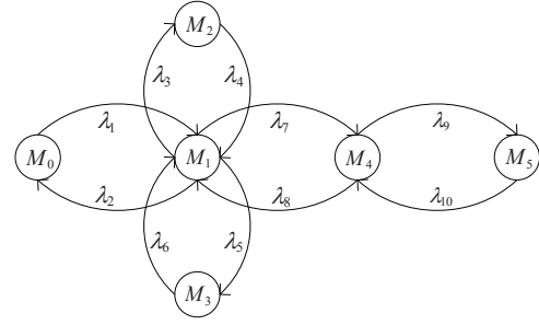
Fig. 6. The equivalent CTMC
