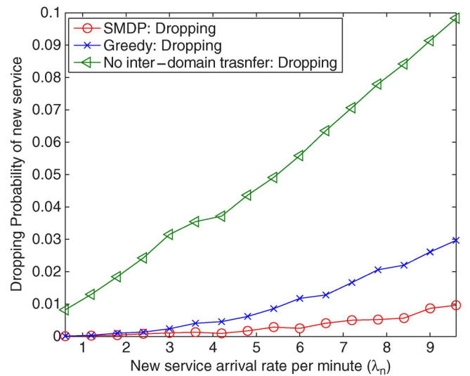
Fig. 8. Dropping probability of new service under various arrival rates ( \lambda_t = 2.4 , \mu_1 = 6.6 , K = 10 ).
