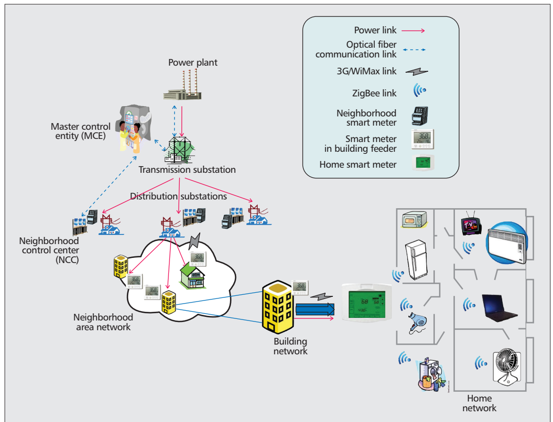
Figure 2. Considered smart grid architecture.
