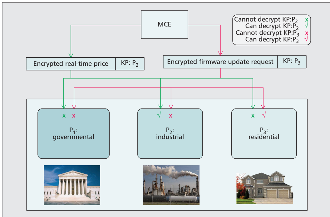
Figure 5. Example of flexible KP-ABE targeted broadcast for real-time price and firmware update request messages.
