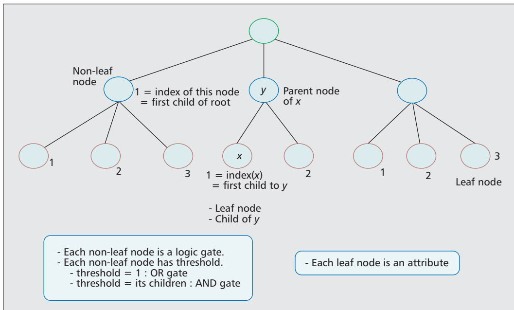
Figure 3. A sample tree-based access structure ( \mathcal{A} ) for KP-ABE in smart grid.
