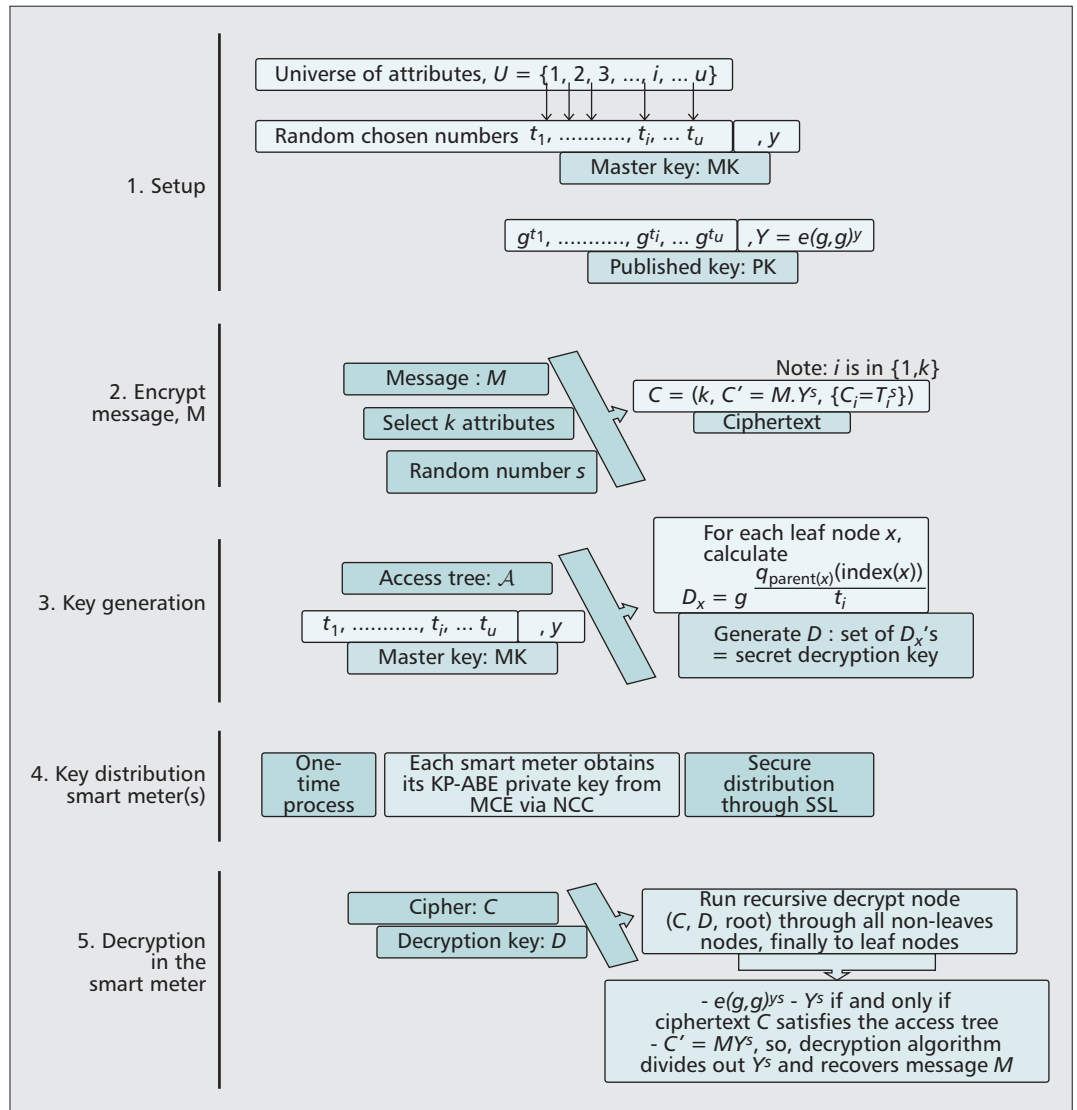
Figure 4. Execution steps of KP-ABE targeted broadcast mechanism in smart grid.
