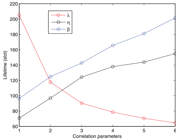
Fig. 5. Network lifetime under different values of \lambda , \eta , and \beta .
