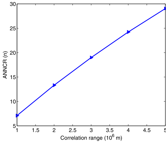
(b) ANNCr Vs. spatial correlation range.
