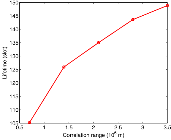
(a) Network lifetime Vs. spatial correlation range.
