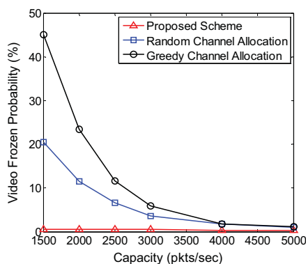
Figure 2 Video frozen probability with different channel allocation schemes in CR network
