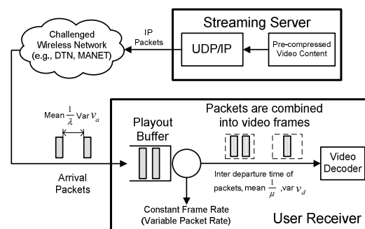
Figure1 Playout Buffer at the Receiver
