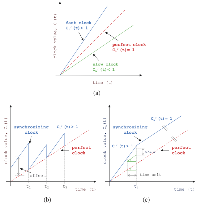
Fig. 2. Clock model. (a) Clock error caused by clocks running at different rates. (b) Offset compensation: clock value is tuned to the clock value of the perfect clock, but the clock offset increases with time due to the clock skew error. (c) Skew compensation: clock frequency is tuned to the clock frequency of the perfect clock, but the clock offset does not match due to the clock offset error.
