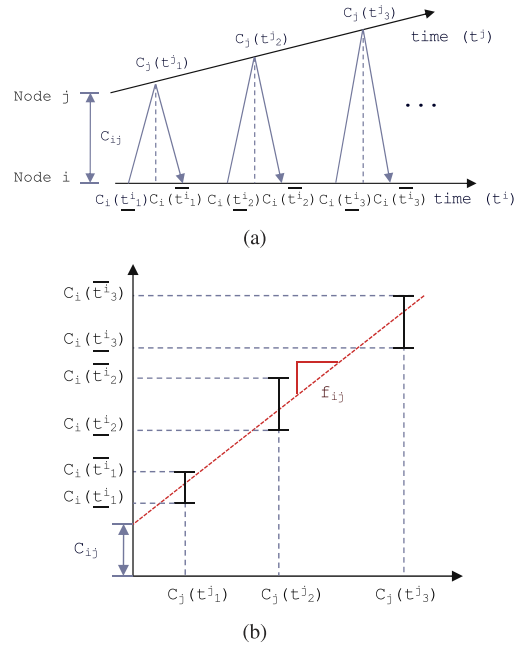
Fig. 3. Relative clock estimation. (a) Exchanging timestamps between nodes i and j . (b) Plotting timestamped triples for clock skew estimation.
