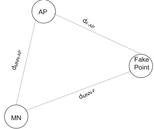
Fig. 5. Fake-point selection.
