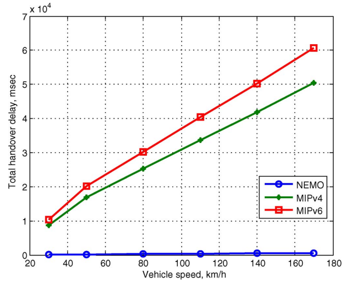
Fig. 17. Total handover delay.
