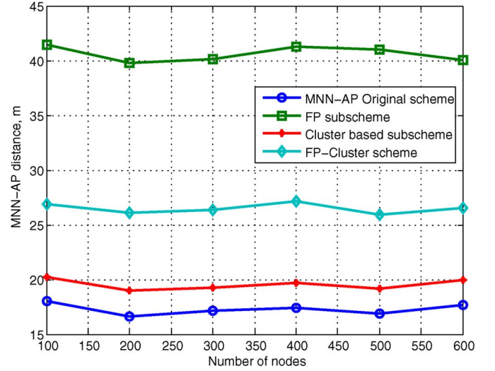
Fig. 13. MNN-AP route distances.
