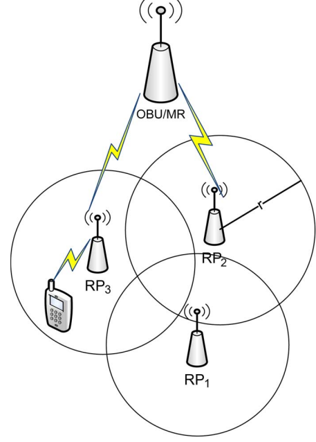
Fig. 7. Cluster-based subscheme.
