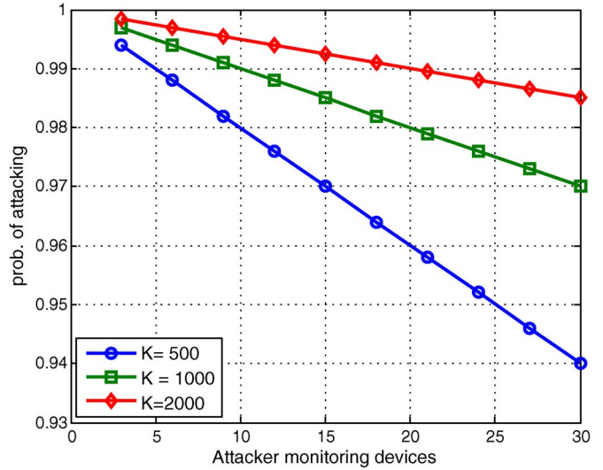
Fig. 8. Fake-point subscheme attacking probability.
