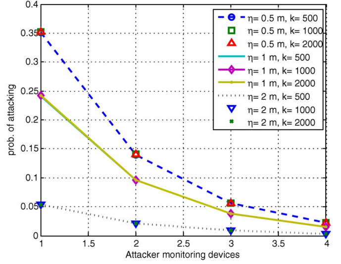
Fig. 10. Fake point-cluster-based scheme attacking probability.
