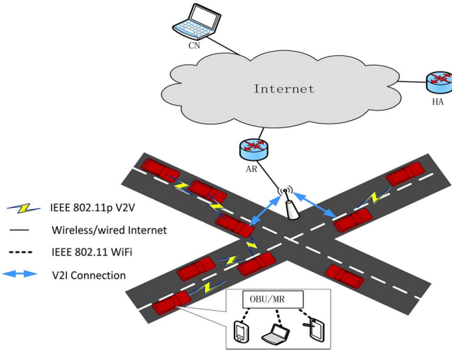
Fig. 1. NEMO-based VANET.
