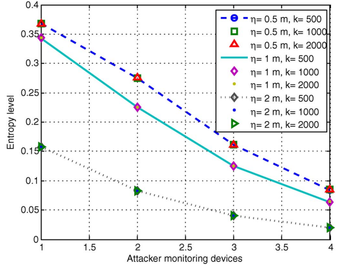
Fig. 11. Fake point-cluster-based entropy.
