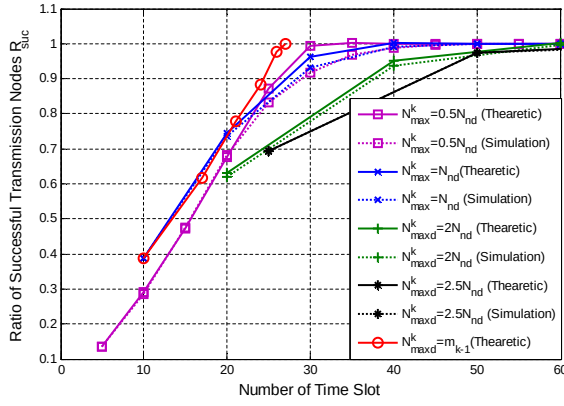
(a) Ratio of successful transmission nodes R_{suc} with N_{nd} = 10 .
