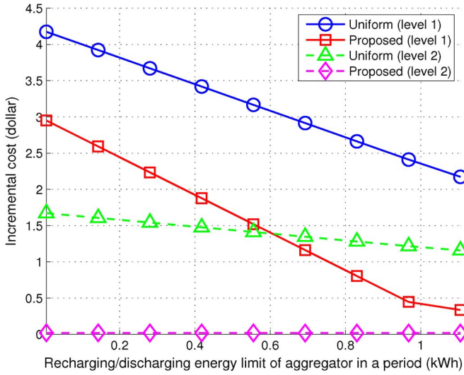
Fig. 7. Incremental cost in a period begins at 4:00 pm.
