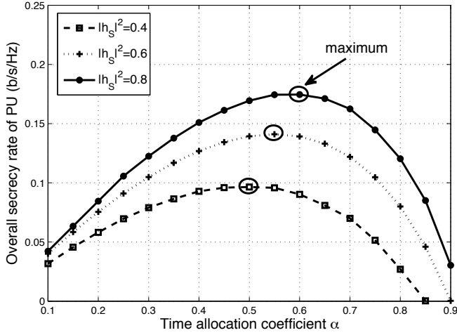
Fig. 3. Overall secrecy rate of PU versus \alpha for R-J scheme for |h_S|^2 = 0.4, 0.6, 0.8 , respectively ( |h_{RD}|^2 = 0.8 , |h_{RE}|^2 = 0.5 , |h_{JD}|^2 = 0.4 , |h_{JE}|^2 = 0.8 , and R_{EX} = 0.4 bit/s/Hz).
