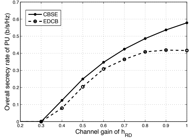
Fig. 7. Comparison between CBSE scheme and EDCB scheme ( |h_{RE}| = 0.3 , |h_{SD}| = 0.3 , |h_{SE}| = 0.4 , N = 3 , and the worst channel |h_{SR,i}|^2 = 0.4 ).
