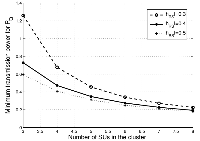
Fig. 12. Minimum transmission power versus the number of SUs for CBNE scheme ( |h_{RD}| = 0.5 , \bar{R}_{EX} = 0.3 b/s/Hz).
