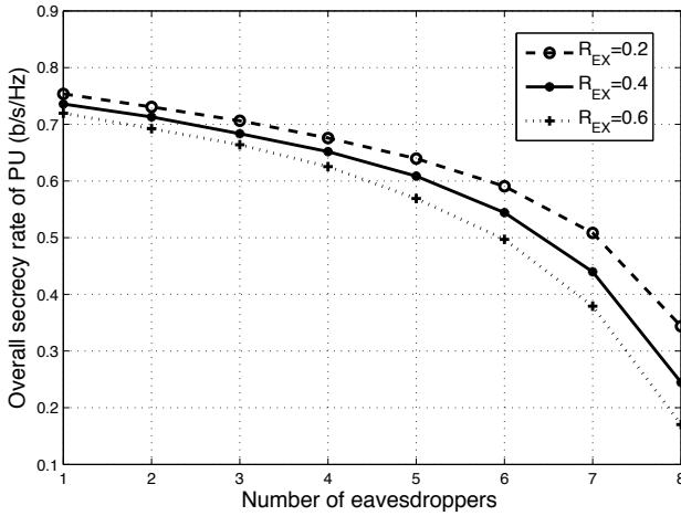
Fig. 10. \bar{R}_{SEC} of PU versus the number of eavesdroppers for CBME scheme ( |h_{RE}| = 0.4 , |h_{RD}| = 0.5 , |h_{RS}| = 0.6 , and N = 10 ).
