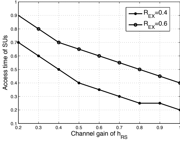
Fig. 5. Access time of SUs versus channel condition h_{RS} for R-J scheme.
