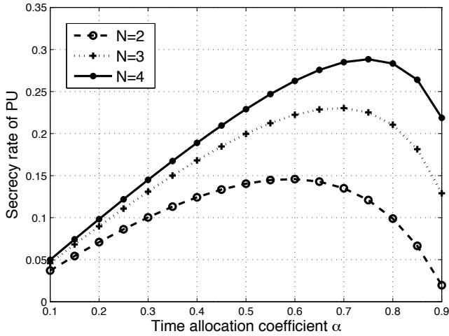
Fig. 6. Overall secrecy rate of the PU versus \alpha for CBSE scheme ( |h_{SD}|^2 = 0.3 , |h_{SE}|^2 = 0.4 , the worst channel |h_{SR,i}|^2 is set to 0.4).
