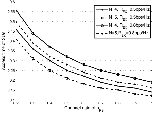
Fig. 9. Access time versus channel condition h_{RS} .
