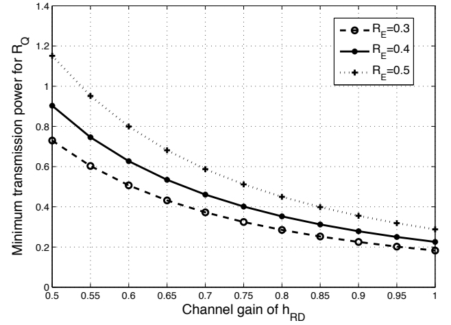
Fig. 11. Minimum transmission power versus |h_{RD}| for CBNE scheme ( |h_{RE}| = 0.4 , |h_{RD}| = 0.5, 0.1 , \bar{R}_Q = 0.5 b/s/Hz and N = 3 ).
