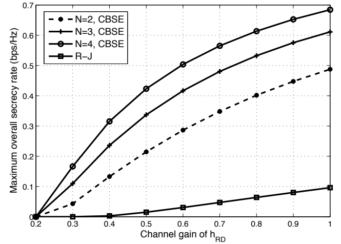
Fig. 8. Comparison between R-J scheme and CBSE scheme.
