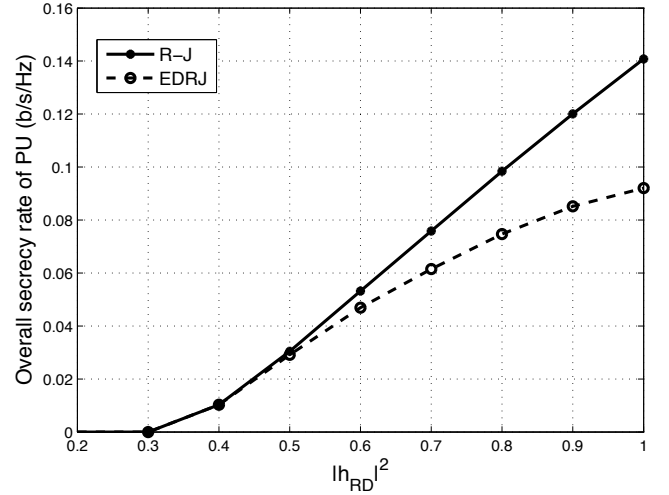
Fig. 4. Comparison between R-J scheme and EDRJ scheme ( |h_{SD}|^2 = 0.3 , |h_{SE}|^2 = 0.4 , |h_{SR}|^2 = 0.6 , |h_{RE}|^2 = 0.3 , |h_{JD}|^2 = 0.3 , and |h_{JE}|^2 = 0.5 ).
