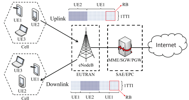
Fig. 1: The architecture of 3GPP LTE network.
