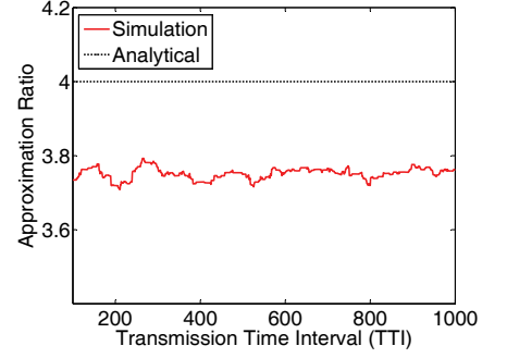
Fig. 6: The approximation ratio between the Optimal and the the Algorithm 2.
