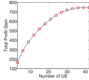
Fig. 3: The numerical example of the Greedy-Downlink algorithm.
