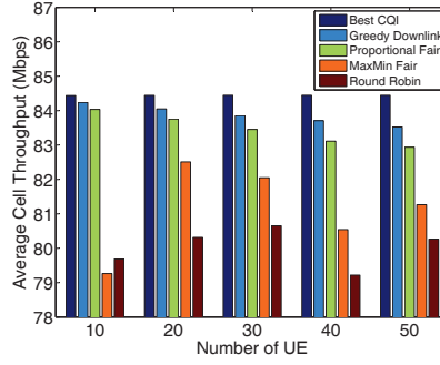
Fig. 5: The average cell throughput of all the downloading UEs. (User speed is 50 km/h.)
