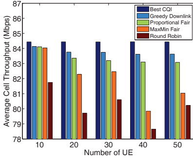
Fig. 4: The average cell throughput of all the downloading UEs. (User speed is 5 km/h.)
