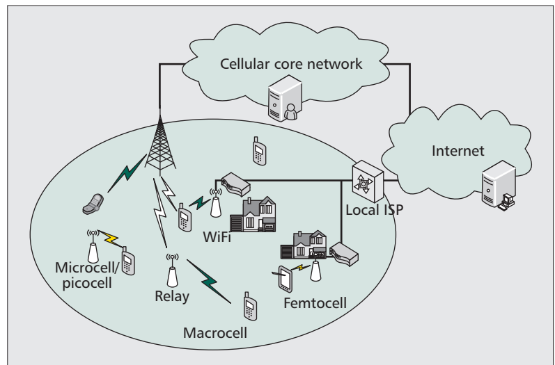
Figure 1. Tiered framework of cognitive cellular networks.
