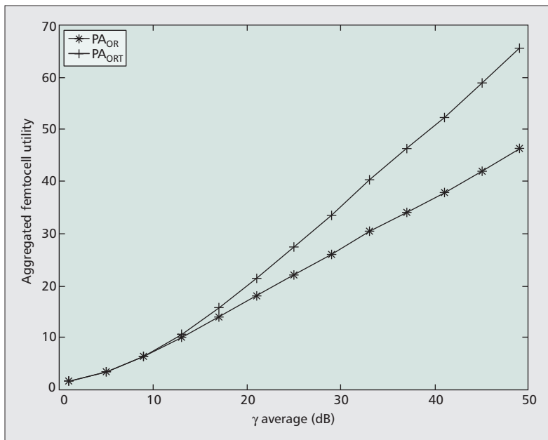
Figure 4. Aggregated femtocell utility under intra-femtocell channel gains.
