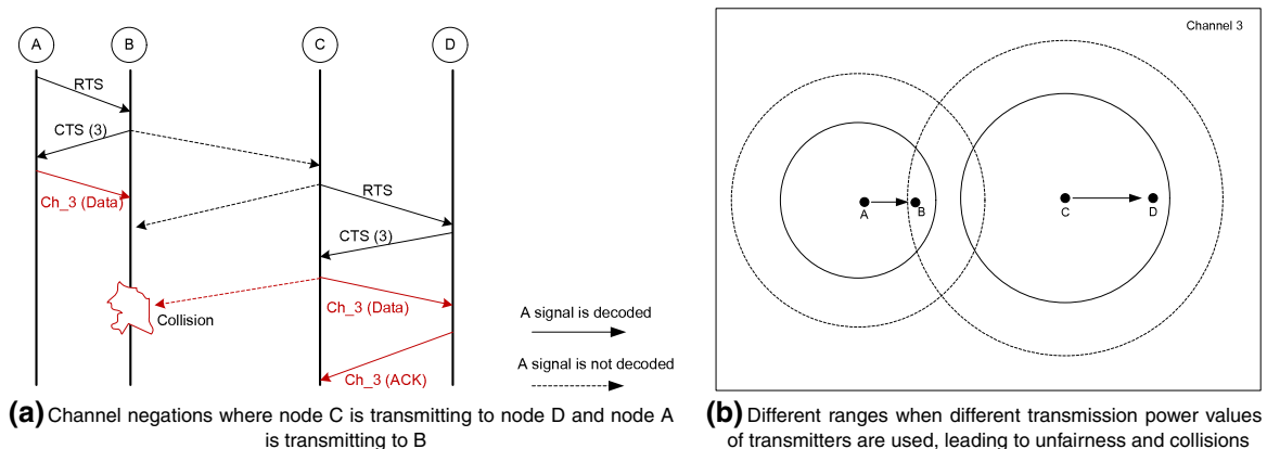
Figure 1. The illustration of the uncontrolled asymmetrical transmission power problem in multi-channel environments.
