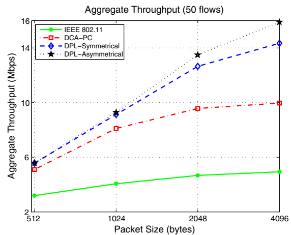
Figure 9. Aggregate throughput versus packet size in the random topology.
