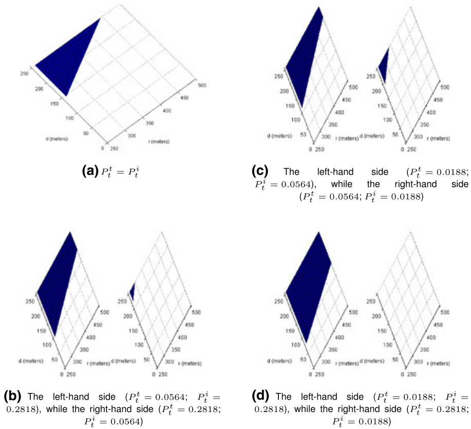
Figure 3. The effect of using different transmission power over a channel. The shadowed areas are the vulnerable areas where collisions occur.
