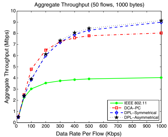
Figure 8. Aggregate throughput in the random topology with different network loads.
