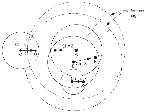
Figure 2. The asymmetrical transmission power can occur without control over multiple channels.
