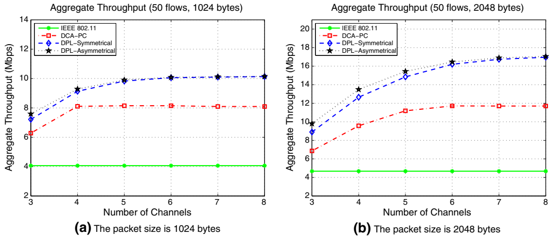
Figure 11. Aggregate throughput versus number of channels in the random topology.
