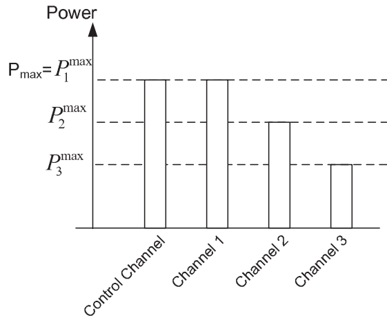
Figure 4. Different allowable powers over different channels.
