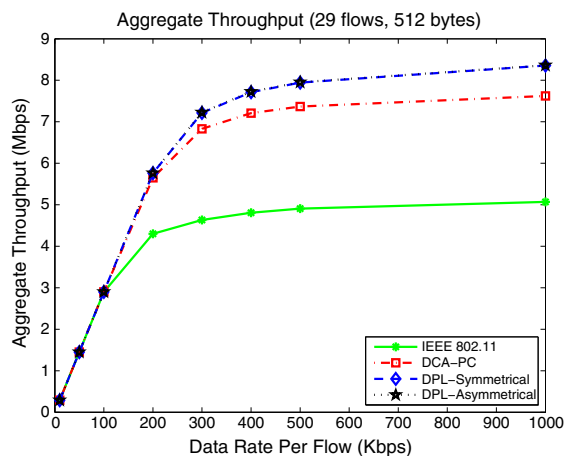
Figure 7. Aggregate throughput in the chain topology with different network loads.
