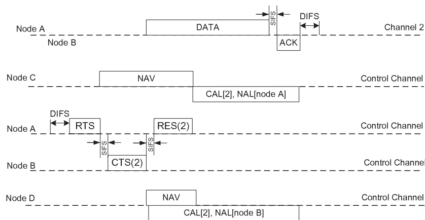
Figure 5. The medium access control protocol using a dedicated control channel and multiple data channels. SIFS, short interframe space; ACK, acknowledgement; DIFS, distributed interframe space; NAV, network allocation vector; RTS, request to send; RES, reservation; CTS, clear to send; CAL, channel allocation list; NAL, node allocation list.
