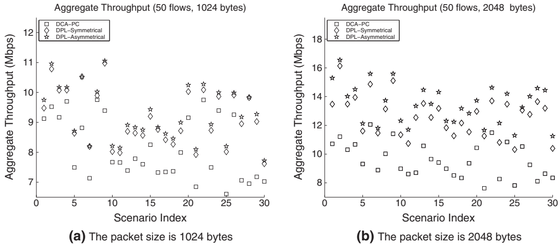
Figure 10. Aggregate throughput of 30 different scenarios in the random topology. DCA-PC, dynamic channel assignment with power control.
