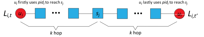
Fig. 7. Linkability of user location information.
