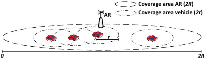
Fig. 1. Asymmetric links in a VANET.
