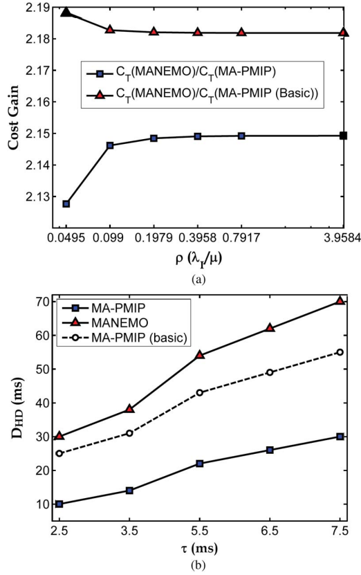
Fig. 8. Cost gain and Handover delay. (a) Cost gain comparison ( 1/\lambda_I = 800 \text{ s} - 10 \text{ s} , v = 50 \text{ Km/h} , S = 300 \text{ B} , and \gamma = 150 \text{ Kb/s} ). (b) Handover delay T_w = 0 \text{ ms} - 5 \text{ ms} , and \delta + S/C = 2.5 \text{ ms} .
