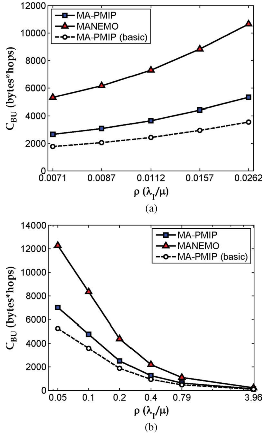
Fig. 6. Location update comparison. (a) Different velocities (1/\lambda_I) = 600 s, and v = 110 Km/h - 30 Km/h. (b) Different session lengths v = 50 Km/h, and (1/\lambda_I) = 800 s - 10 s.
