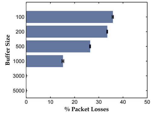
Fig. 13. MA-PMIP packet losses due to buffer overflow.
