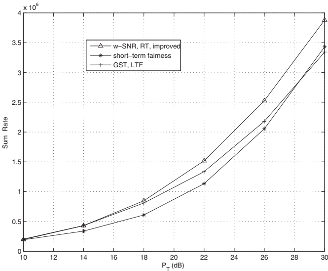
Fig. 11. Sum rates vs. transmit power P_T for the adaptive w -SNR, short-term fairness, and GST schemes in uplink OFDMA, with K = 4 , N = 32 , unequal target BERs, unequal channel ASNRs, \alpha = [1 : 1 : 1 : 1] , \tilde{R}_{\min} = 0 bits/s/Hz, P_{T,k} = P_T/K for all k , and L = 8 paths with an exponentially decayed PDP.
