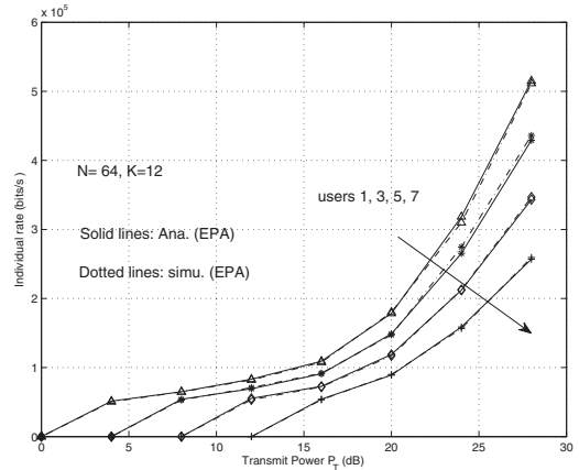
Fig. 5. Analytical and simulated individual rates vs. transmit power P_T for the optimal w -SNR scheme with EPA in downlink OFDMA, with K = 12 , N = 64 , unequal target BERs, unequal channel ASNRs, \alpha = [12 : 11 : \dots : 1] , with the minimum link-rate constraint ( \tilde{R}_{\min} = 2 bits/s/Hz), and L = 8 paths with an exponentially decayed PDP.
