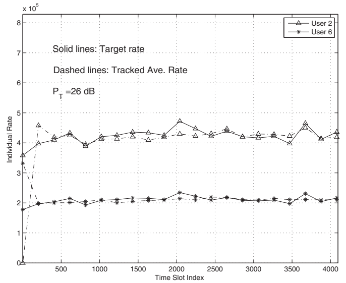
Fig. 12. Individual tracked and targets rates vs. time for the adaptive w -SNR scheme in uplink OFDMA, with K = 8 , N = 32 , P_T = 26 dB, unequal target BERs, unequal channel ASNRs, \alpha = [2 : 2 : 2 : 2 : 2 : 1 : 1 : 1 : 1] , \tilde{R}_{\min} = 1 bits/s/Hz, P_{T,k} = P_T/K for all k , and L = 8 paths with an exponentially decayed PDP.
