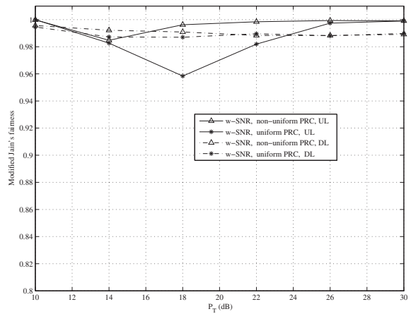
Fig. 13. Modified Jain's fairness metric vs. transmit power P_T for the adaptive w -SNR schemes in uplink and downlink OFDMA systems, with K = 8 , N = 32 , unequal target BERs, unequal channel ASNRs, with uniform and non-uniform target rate proportions, and L = 8 paths with an exponentially decayed PDP.
