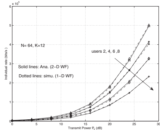
Fig. 2. Analytical and simulated individual rate vs. P_T in downlink OFDMA of users 2,4,6,8 with 1-D and 2-D WF power allocation of the optimal w -SNR scheme, with K = 12 , N = 64 , unequal target BERs, equal channel ASNRs, \alpha = [12 : 11 : \dots : 2 : 1] , without the minimum link-rate constraint. L = 8 paths with an exponentially decayed PDP.
