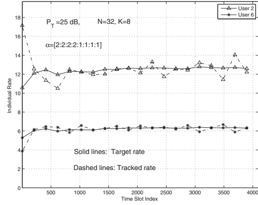
Fig. 8. Individual tracked and targets rates vs. time for the adaptive w -SNR scheme in downlink OFDMA, with K = 8 , N = 32 , P_T = 25 dB, unequal target BERs, unequal channel ASNRs, \alpha = [2 : 2 : 2 : 2 : 1 : 1 : 1 : 1] , \tilde{R}_{\min} = 2 bits/s/Hz, and L = 8 paths with an exponentially decayed PDP.
