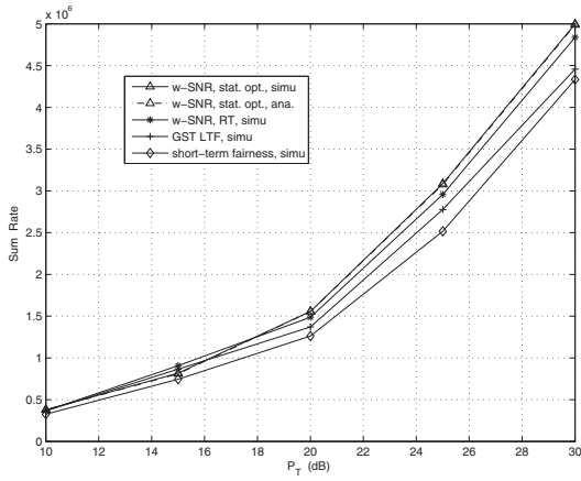
Fig. 6. Analytical and simulated sum rates vs. transmit power P_T for the w -SNR, the STF, and LTF GST schemes in downlink OFDMA, with K = 8 , N = 32 , unequal target BERs, unequal channel ASNRs, \alpha = [2 : 2 : 2 : 2 : 1 : 1 : 1 : 1] , \tilde{R}_{\min} = 2 bits/s/Hz, and L = 8 paths with an exponentially decayed PDP.
