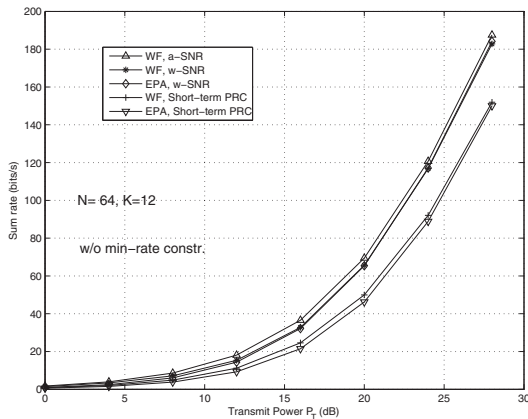
Fig. 1. Simulated sum rates vs. transmit power P_T for the proposed w -SNR and others schemes in downlink OFDMA, with K = 12 , N = 64 , unequal target BERs, equal channel ASNRs, \alpha = [12 : 11 : \dots : 2 : 1] , without the minimum link-rate constraint. L = 8 paths with an exponentially decayed PDP.
