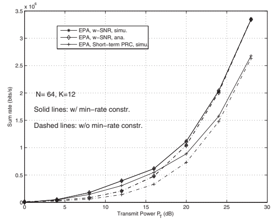
Fig. 4. Analytical and simulated sum rates vs. transmit power P_T for the optimal w -SNR scheme and the short-term fairness scheme in downlink OFDMA, with K = 12 , N = 64 , unequal target BERs, unequal channel ASNRs, \alpha = [12 : 11 : \dots : 2 : 1] , with and without the minimum link-rate constraint ( \tilde{R}_{\min} = 2 bits/s/Hz or 0), and L = 8 paths with an exponentially decayed PDP.
