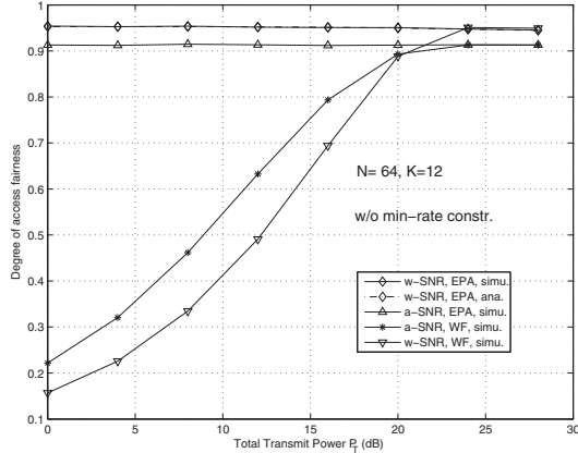
Fig. 3. Degree of access fairness vs. P_T in downlink OFDMA of the w -SNR and the a -SNR schemes, with K = 12 , N = 64 , unequal target BERs, equal channel ASNRs, \alpha = [12 : 11 : \dots : 2 : 1] , without the minimum link-rate constraint. L = 8 paths with an exponentially decayed PDP.
