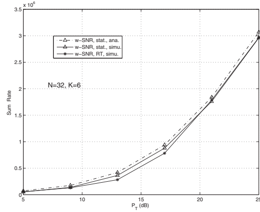
Fig. 9. Sum rates vs. transmit power P_T for the w -SNR schemes with statistical w and adaptive w , respectively, in uplink OFDMA, with K = 6 , N = 32 independent subchannels, unequal target BERs, equal channel ASNRs, \alpha = [2 : 2 : 2 : 2 : 1 : 1 : 1 : 1] , \tilde{R}_{\min} = 0 , and P_{T,k} = P_T/K for all k .
