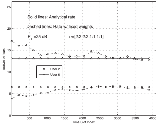
Fig. 7. Individual tracked and analytical rates vs. time for the optimal w -SNR scheme in downlink OFDMA, with K = 8 , N = 32 , P_T = 25 dB, unequal target BERs, unequal channel ASNRs, \alpha = [2 : 2 : 2 : 2 : 1 : 1 : 1 : 1] , \tilde{R}_{\min} = 2 bits/s/Hz, and L = 8 paths with an exponentially decayed PDP.
