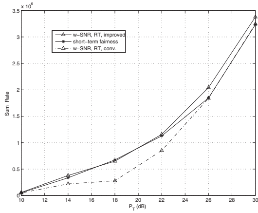
Fig. 10. Sum rates vs. transmit power P_T for the adaptive w -SNR and short-term fairness schemes in uplink OFDMA, with K = 8 , N = 32 , unequal target BERs, unequal channel ASNRs, \alpha = [1 : 1 : 1 : 1 : 1 : 1 : 1 : 1] , \tilde{R}_{\min} = 1 bits/s/Hz, P_{T,k} = P_T/K for all k , and L = 8 paths with an exponentially decayed PDP.
