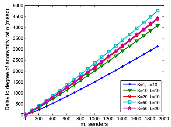
Figure 10. Mix-based's delay-to-degree of anonymity ratio.
