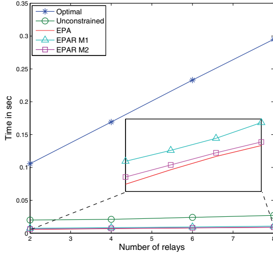
Fig. 12. Average running time for K = 16 , where 8 GBR users with equal rate requirements of 3 bits/sec/Hz.
