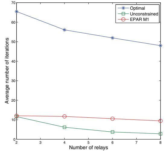
Fig. 11. Average number of iterations for converging all dual variables with K = 16 , where 8 GBR users with equal rate requirements of 3 bits/sec/Hz.
