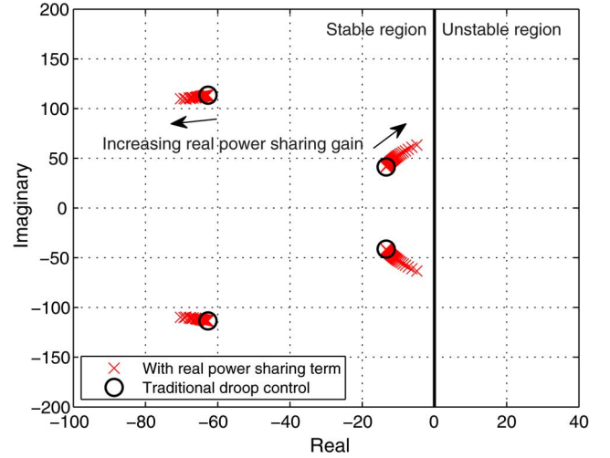
Fig. 4. Trace of low-frequency modes versus real power sharing gain.
