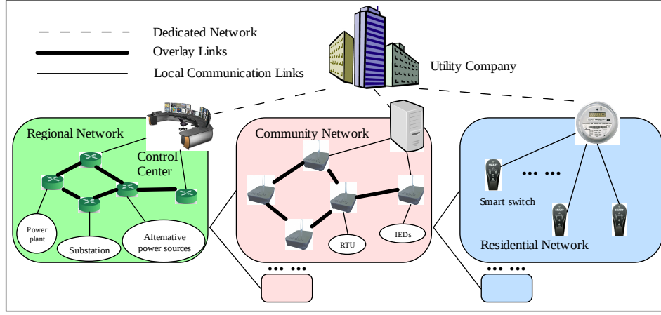
Fig. 1. Network architecture for smart grid
