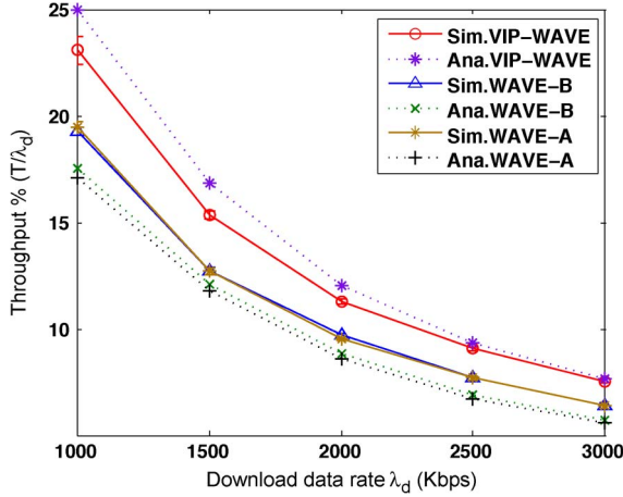
Fig. 13. Nodal downstream throughput under saturated conditions for highly demanding IP applications, RSU interdistance X = 1500 m, average speed v = 35 Km/h, and constant density \rho = 1/25 vpm.
