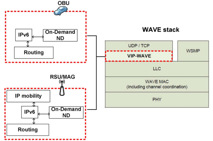
Fig. 4. VIP-WAVE architecture.
