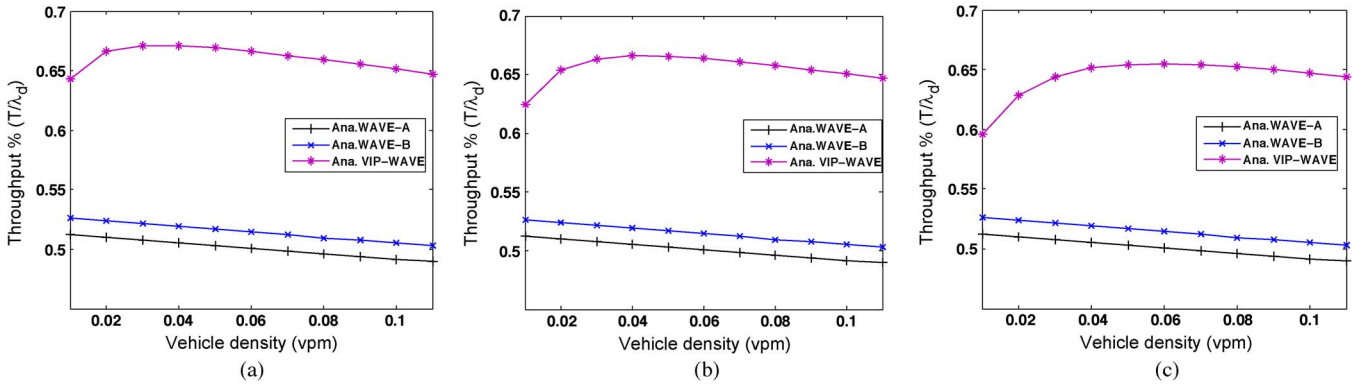
Fig. 12. Nodal downstream throughput for different vehicle densities, RSU interdistance X = 1500 m, and average speed v = 35 Km/h. (a) p_r = 1.0 . (b) p_r = 0.7 . (c) p_r = 0.4 .
