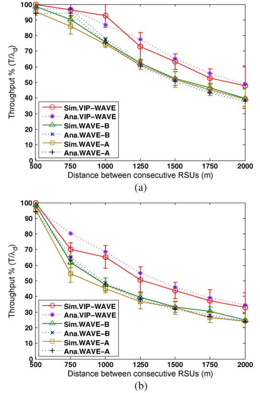
Fig. 9. Nodal downstream throughput for different levels of presence of infrastructure, average speed v = 35 Km/h, constant density \rho = 1/25 vpm, and p_r = 0.4 . (a) One-way traffic. (b) Two-way traffic.
