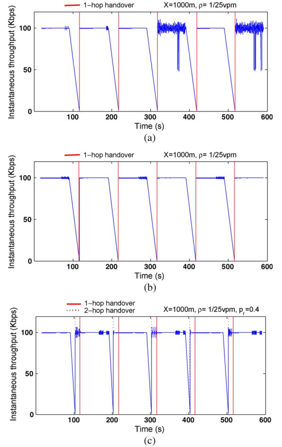
Fig. 14. Instantaneous throughput and handover delay for different WAVE schemes. (a) WAVE-A. (b) WAVE-B. (c) VIP-WAVE.
