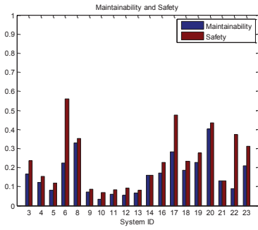
Fig. 8. Maintainability and safety of LANL systems
