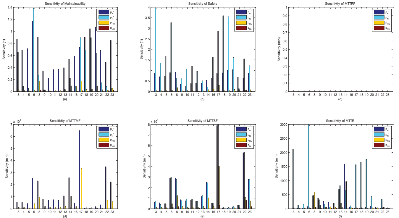
Fig. 12. Transition probability parameter sensitivity analysis
