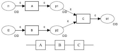
Fig. 7(c). Synchronization pattern
