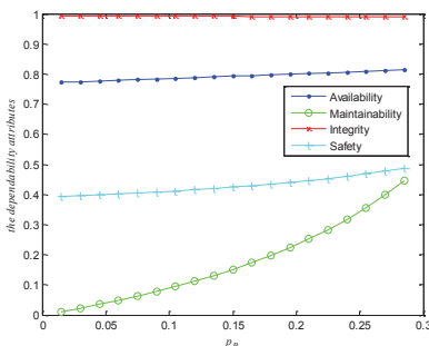
Fig. 4. Dependability with different p_R
