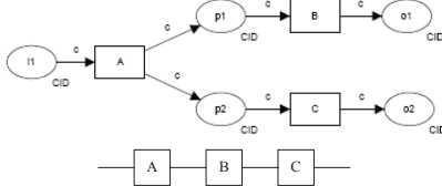
Fig. 7(b). Parallel split pattern
