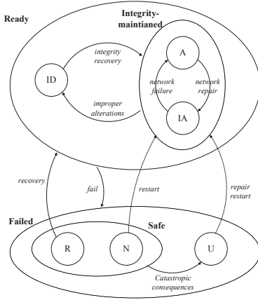
Fig. 2. A state transition graph for services computing systems
