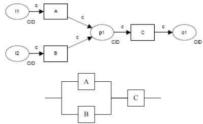
Fig. 7(e). Simple merge pattern
