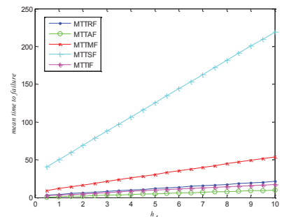
Fig. 6. MTTFs with different h_A
