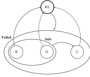
Fig. 3. Simplified SMP model
