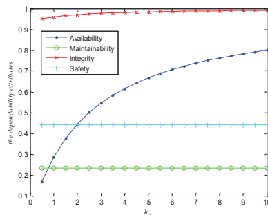
Fig. 5. Dependability with different h_A
