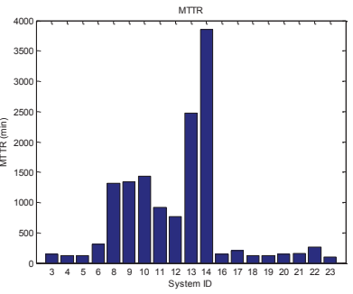
Fig. 10. MTTR of LANL systems
